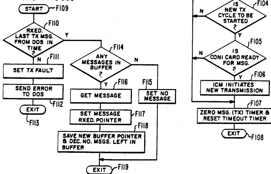
FIG. 30 DOS REQUESTS ICM TO INPUT DATA TO DOS
