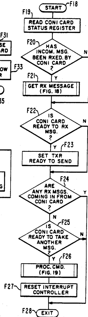
FIG. 26 CONI CARD INTERRUPT
