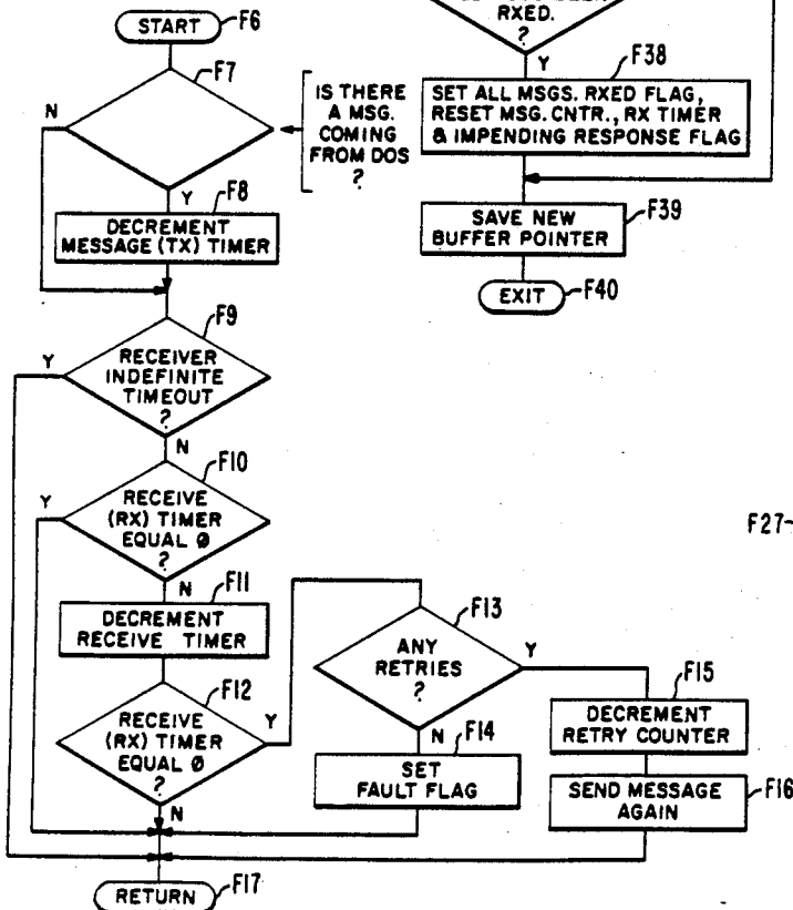
FIG. 27 INCOM DRIVER TIMER TICK INTERRUPT SERVICE ROUTINE
