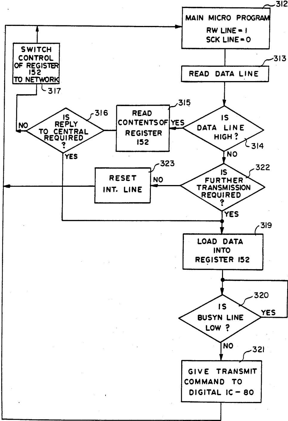
FIG. 23 INTERFACE FLOW CHART FOR MICROCOMPUTER - 84
