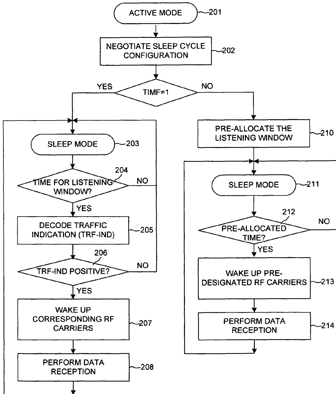
POWER MANAGEMENT FLOW CHART FOR SLEEP MODE OPERATION
