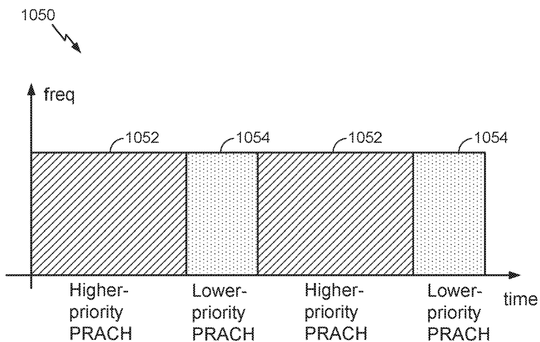
PRACH resources for one configuration
