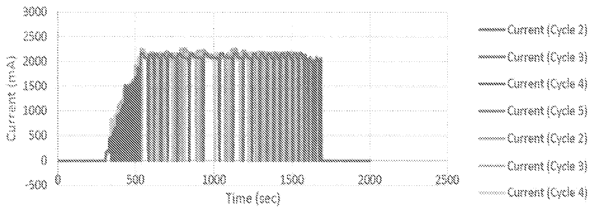
Current vs Time During a Number of Charge Cycles using NLV
