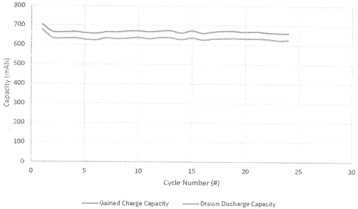
Charge Capacity & Discharge Capacity vs Cycle Number During NLV Based Charging, Avg Charge Time @ 23.45 Mins
