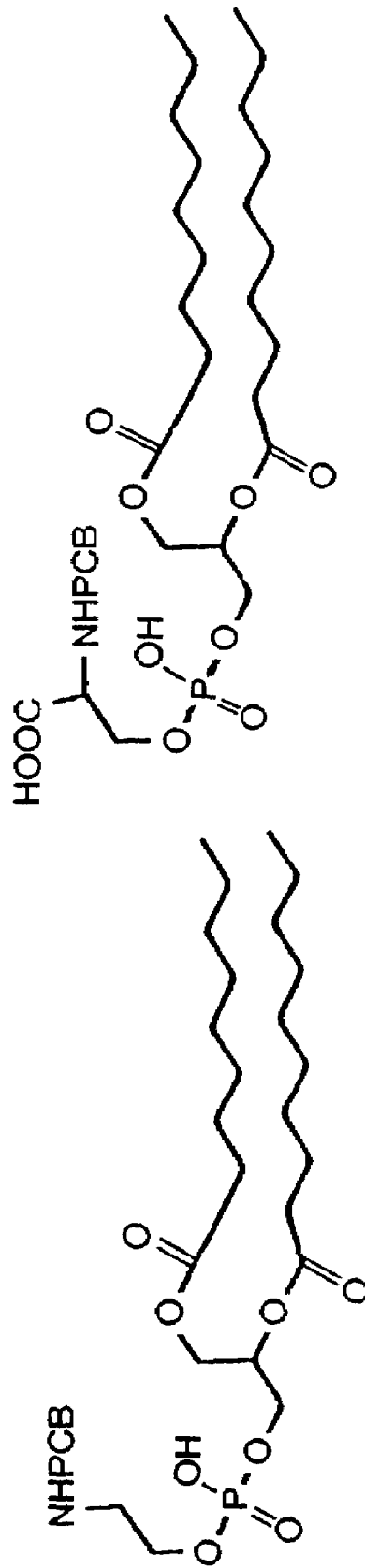
PCB-Phosphatidylethanoamine (PCB-PE)
