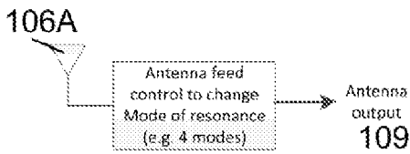
Donor Antenna Sub-system 105B
