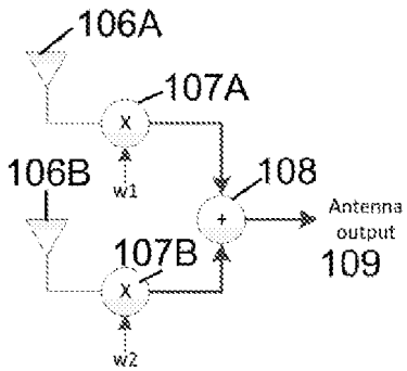
Donor Antenna Sub-system 105A
