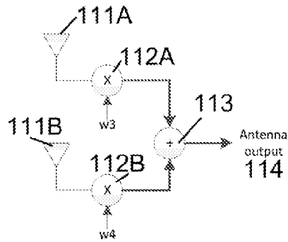
Server Antenna Sub-system 110A
