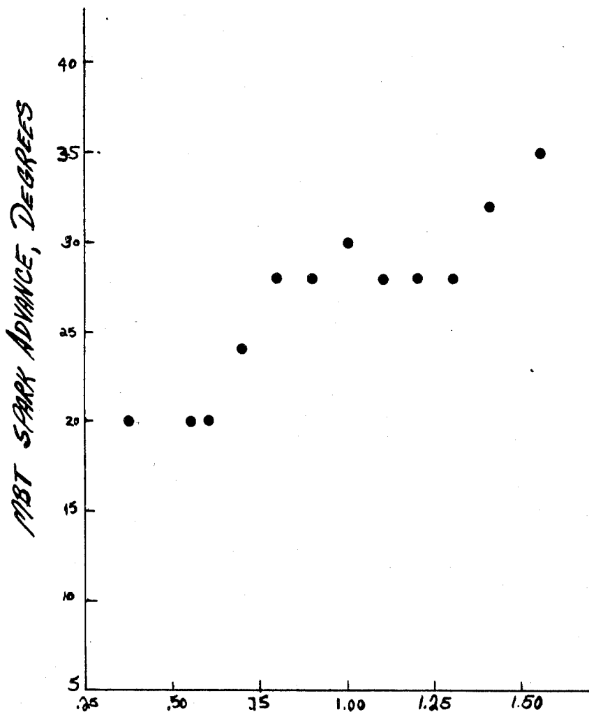
FLAP OPENING, IN. HIGH LOAD FLAP SENSITIVITY TEST ( \approx 105 IMEP) FIG. 68 (ER-709) (DECEMBER 29, 1977 DATA)
