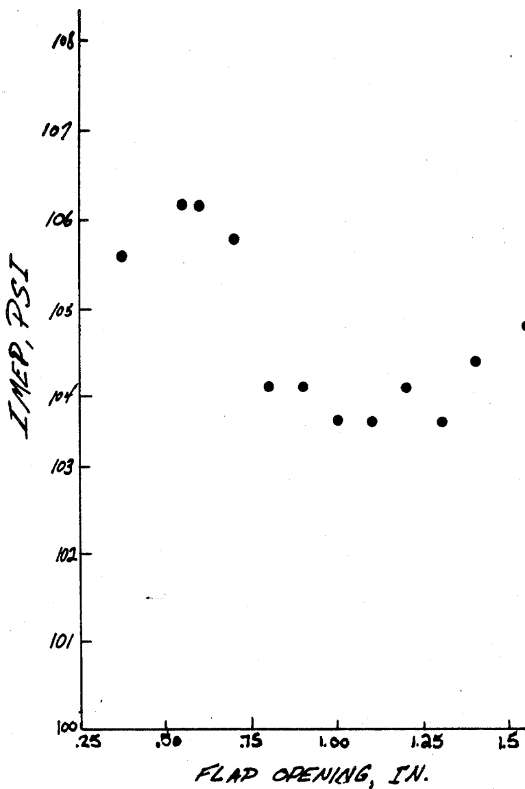
HIGH LOAD FLAP SENSITIVITY TEST FIG. 69 (ER: .709) (MST SPARK ADVANCE) (DECEMBER 29, 1977 DATA)
