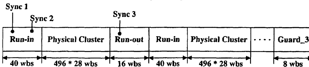
Continuously written sequence of Recording Unit Blocks
