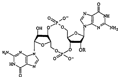
c-G(2'-OR)pGp R = CH 3 , C 2 H 5 , etc. (III)
