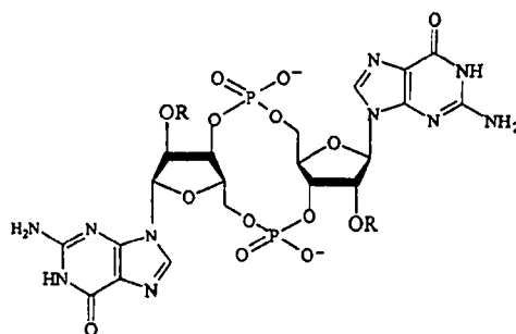
c-G(2'-OR)pG(2'-OR)p R = CH 3 , C 2 H 5 , etc. (IV)
