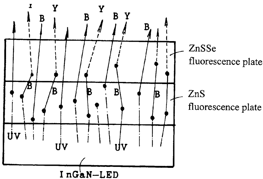
ultraviolet type white color light emitting device Q
