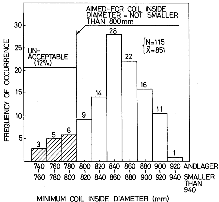
FIG. 3 PRIOR ART
