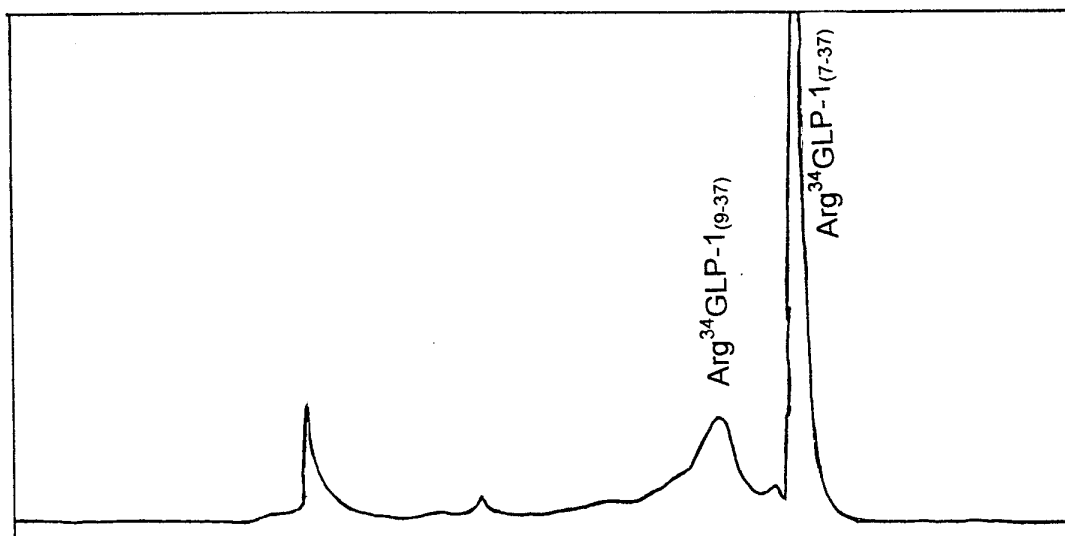
Chromatogram of Example 10.
