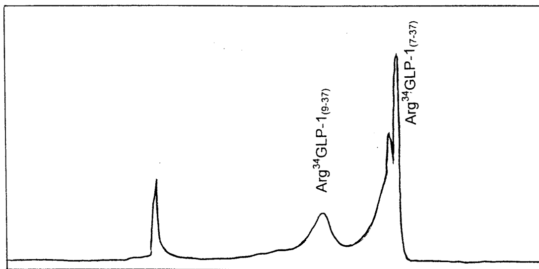
Chromatogram of Example 11.
