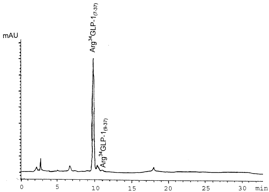
Analytical chromatogram of Example 1. Eluate.
