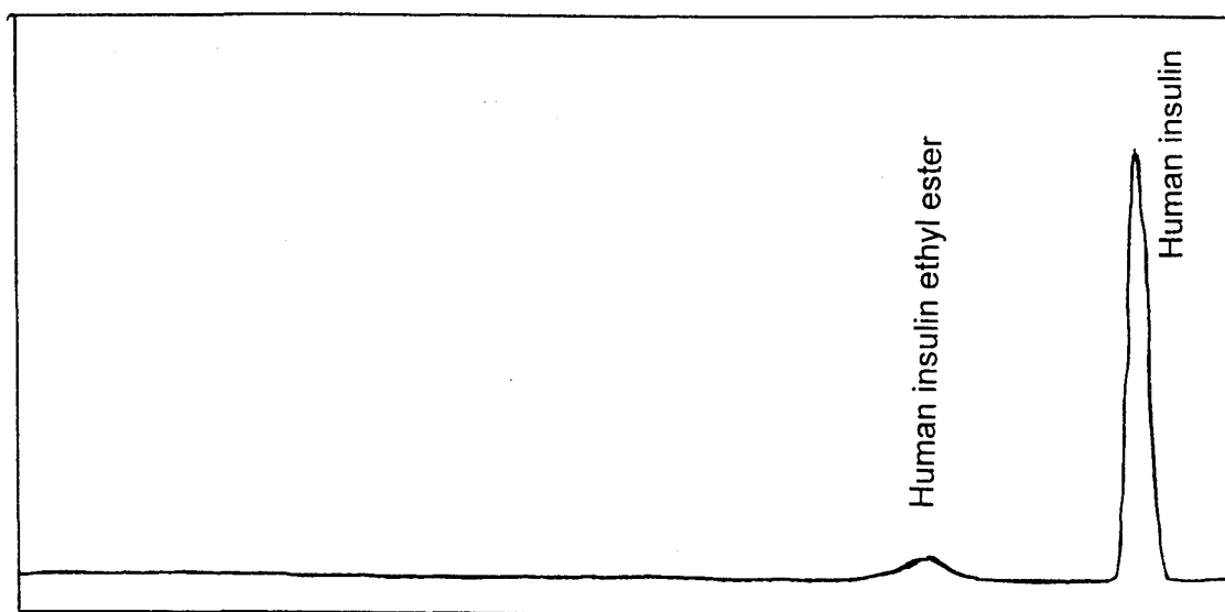
Chromatogram of Example 14.
