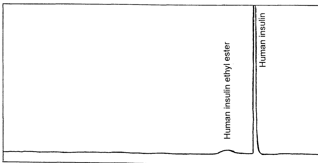
Chromatogram of Example 16.
