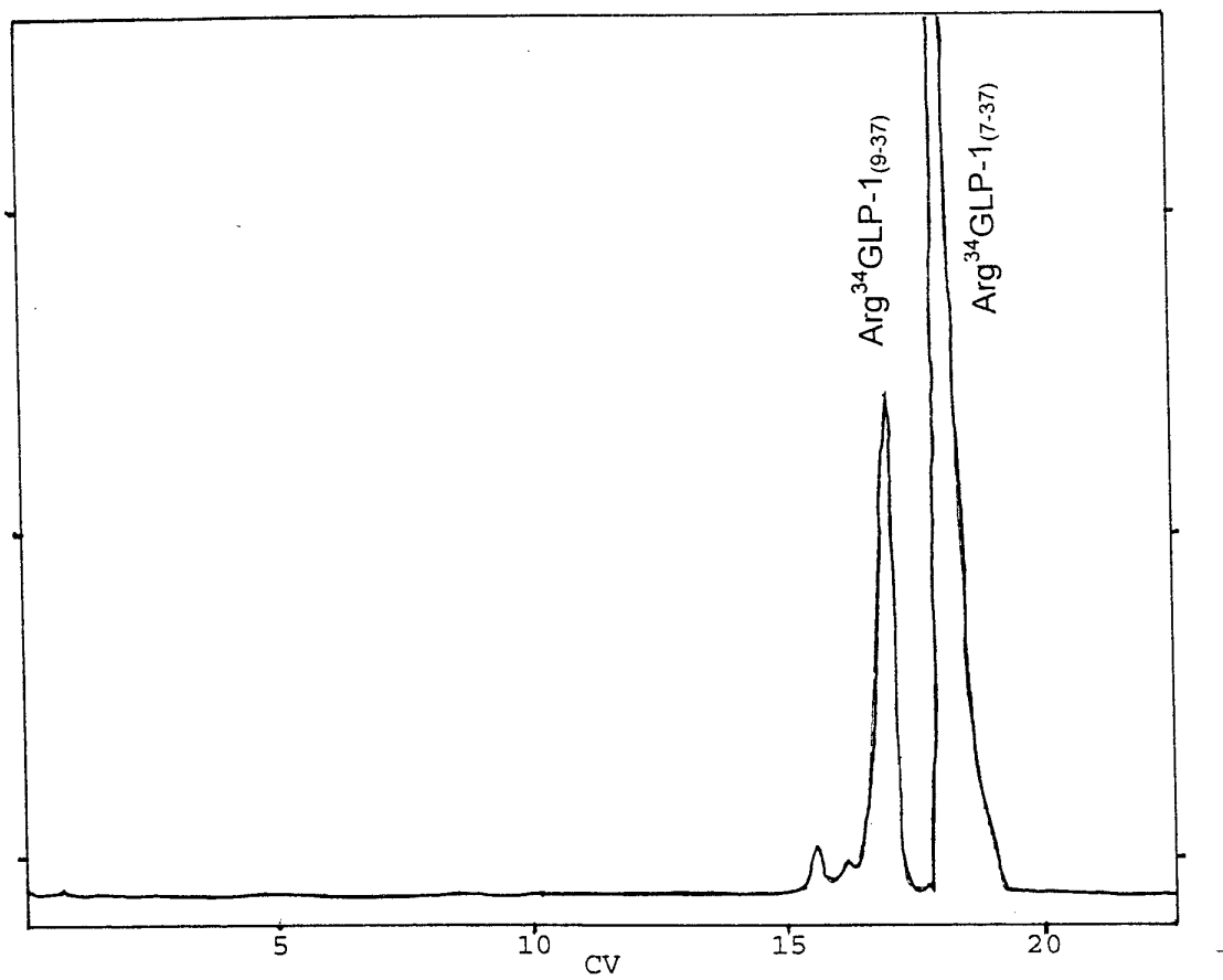
Chromatogram of Example 3.
