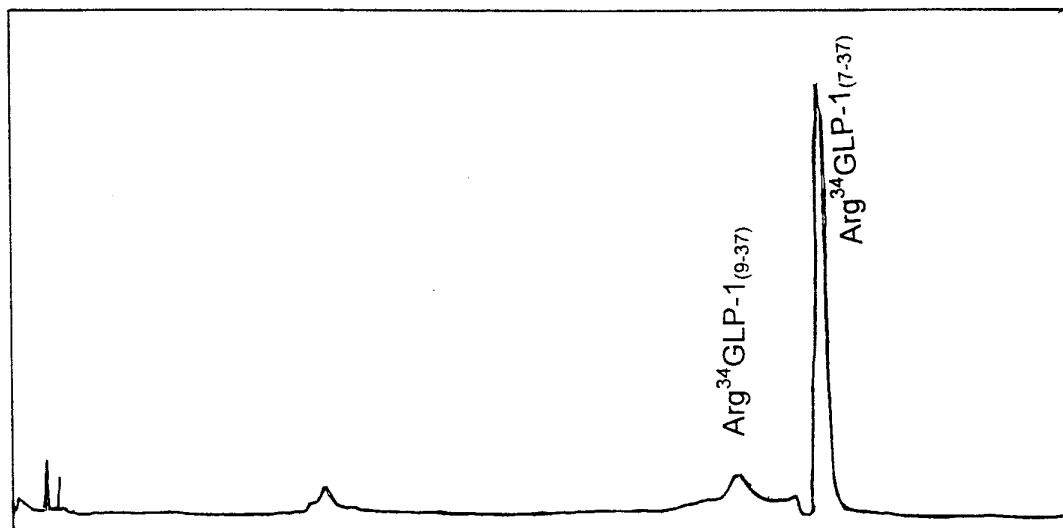
Chromatogram of Example 5.
