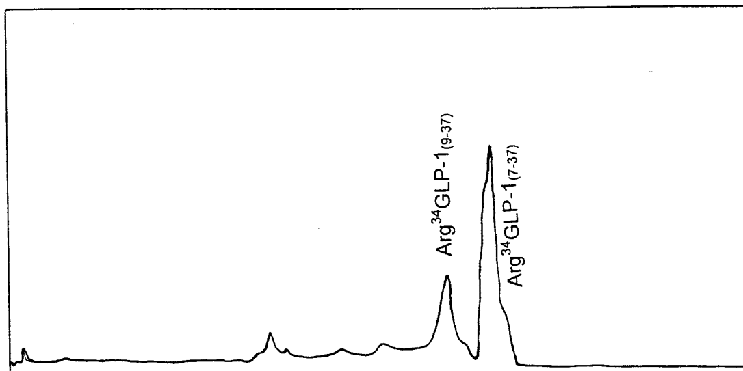
Chromatogram of Example 12.
