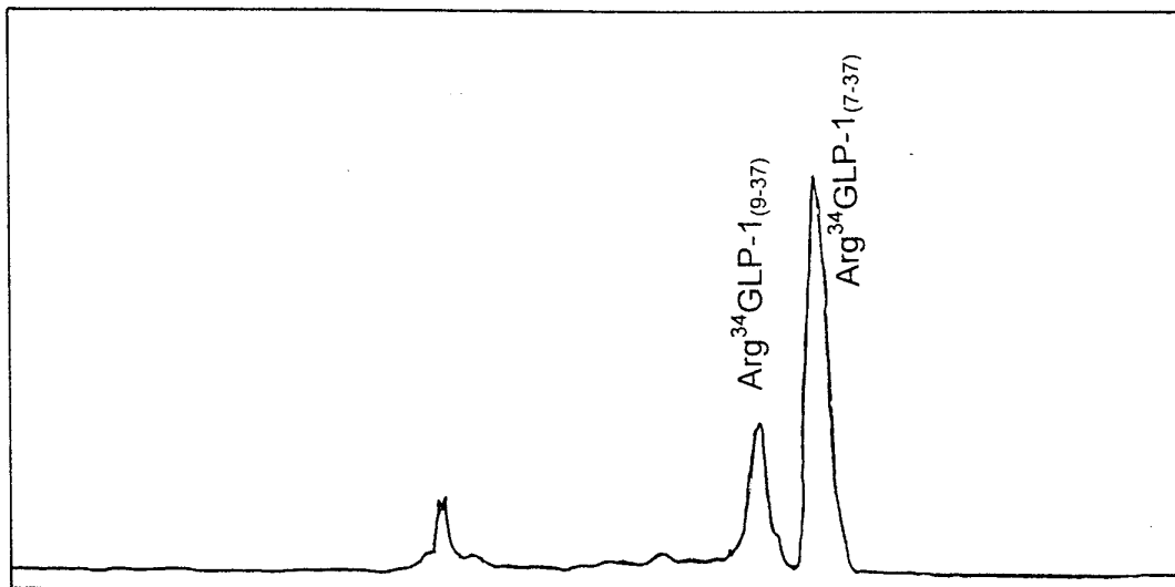
Chromatogram of Example 9.
