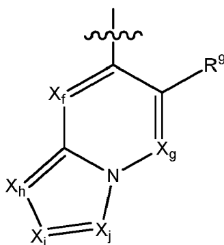
Formula C
