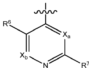
Formel A
