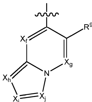
Formel C
