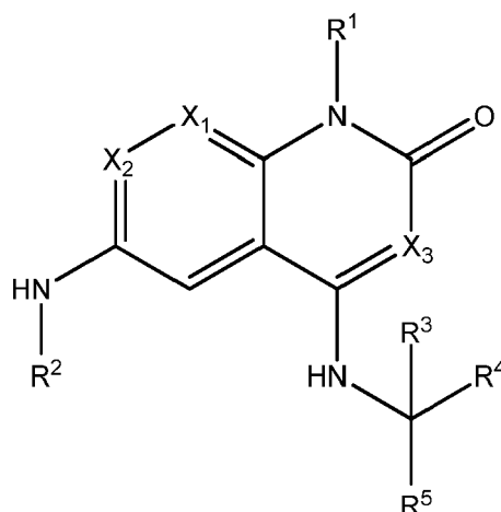
Formel (I)
