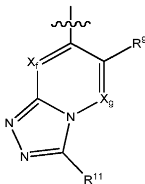
Formula C
