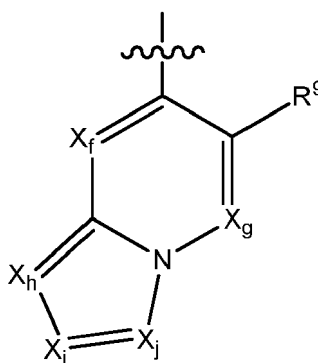
Formel C
