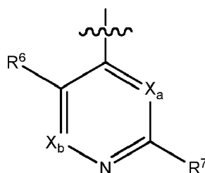
Formula A
