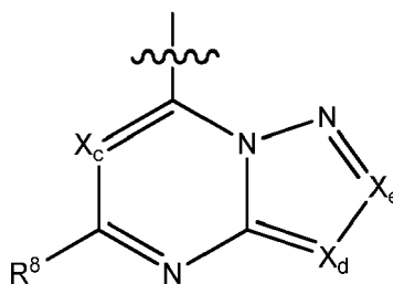
Formel B
