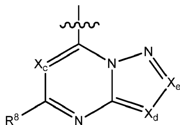
Formula B
