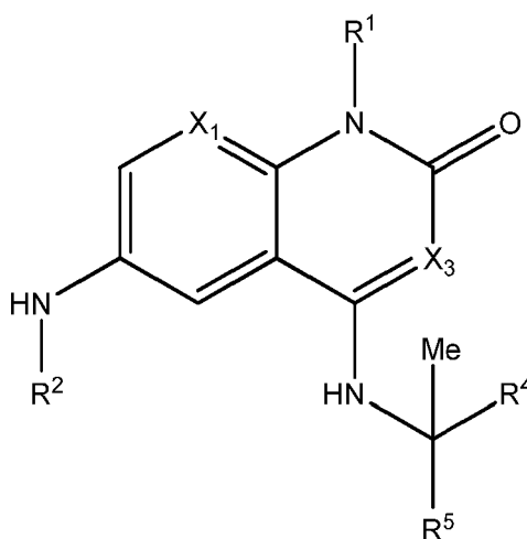
Formel Ib 2
