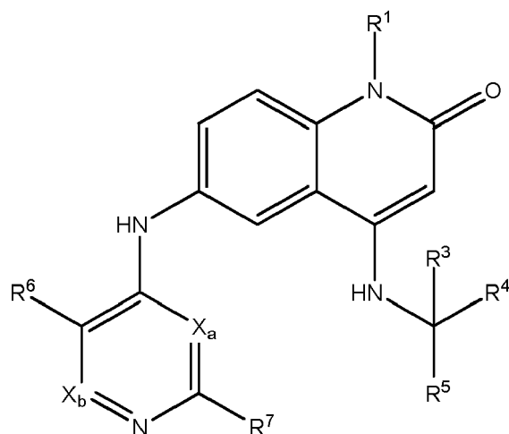
Formula If
