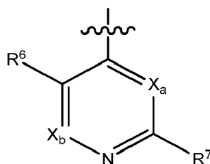
Formel A
