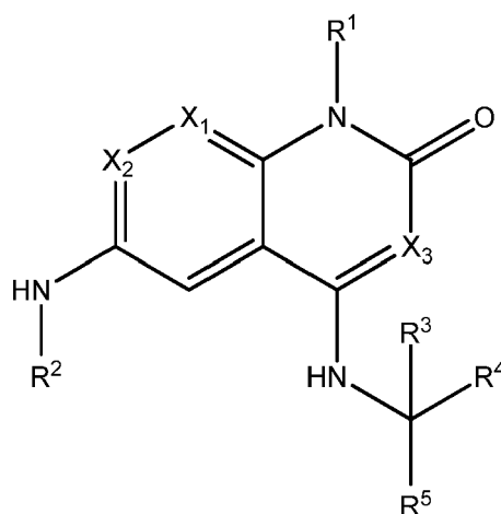
Formula (I)
