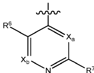
Formula A
