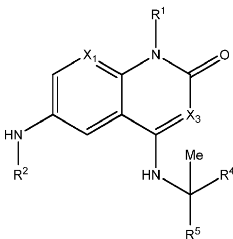
Formula Ib 2
