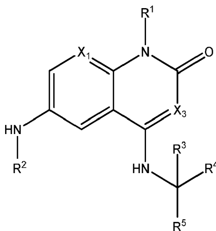
Formula Ia
