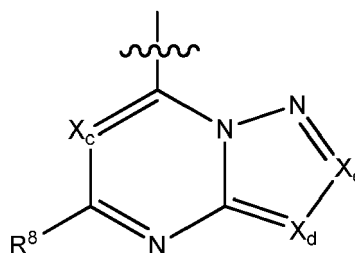
Formel B
