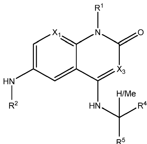
Formula Ib
