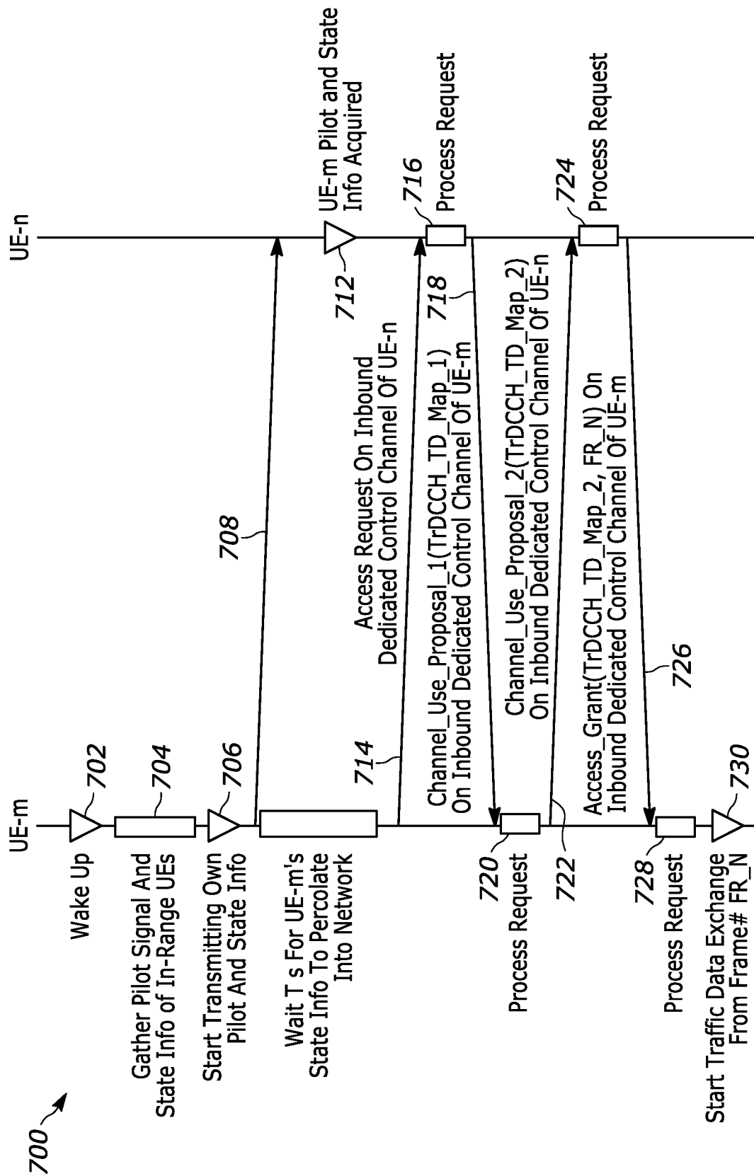
Bi-Directional Link Establishment From UE Wake Up
