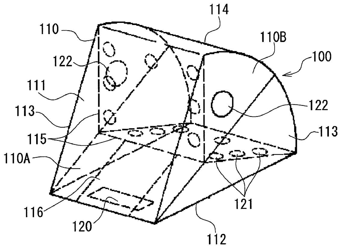
FIG. 22 Prior Art
