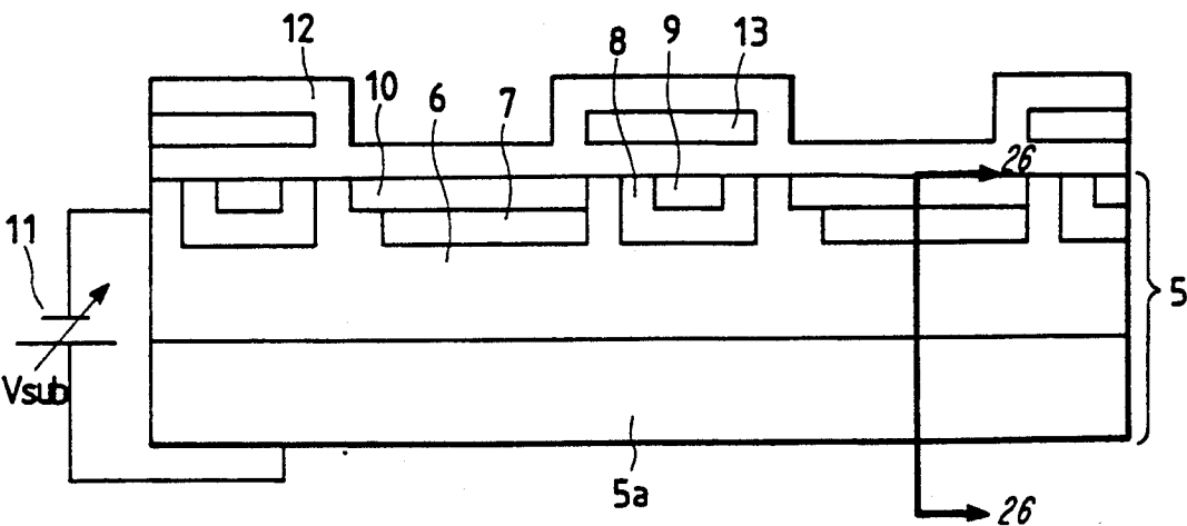
FIG. 25 PRIOR ART
