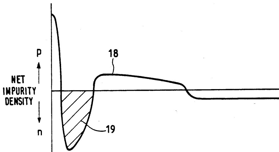
FIG. 27 PRIOR ART
