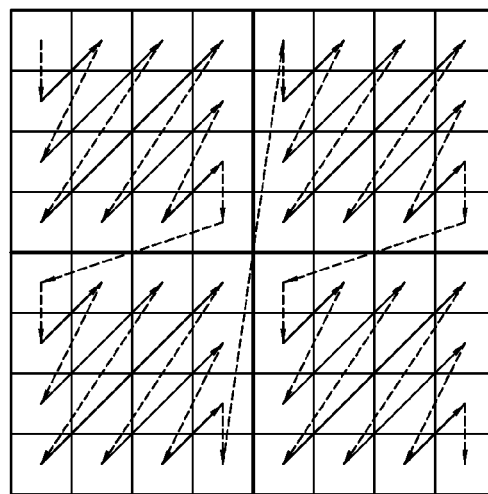
diagonal scanning (860)
