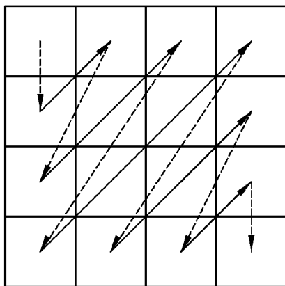
diagonal scanning (840)
