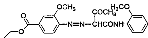
Formula (13)
