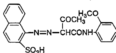
Formula (5)
