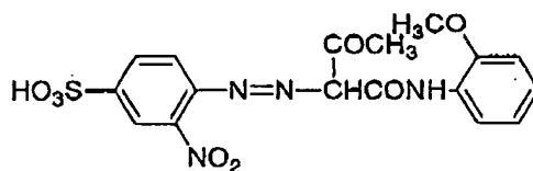
Formula (8)
