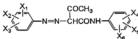
Formula (1)
