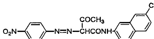
Formula (23)
