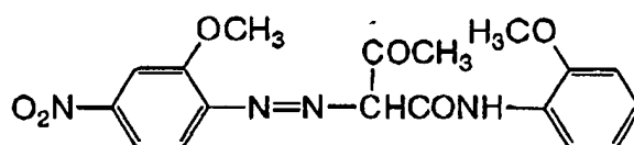
Formula (2)
