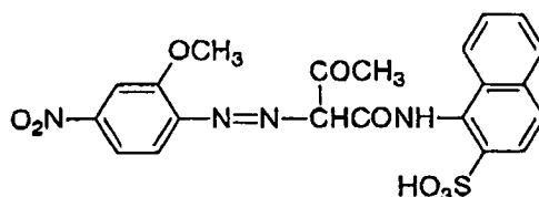
Formula (21)
