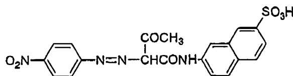
Formula (20)
