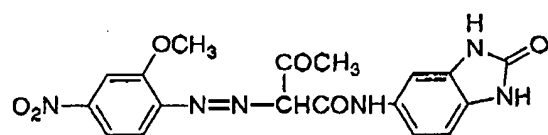
Formula (15)
