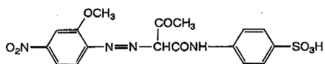
Formula (16)
