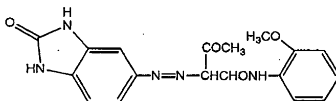
Formula (25)
