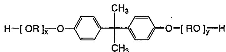
Formula (3)
