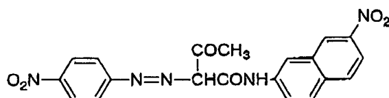
Formula (22)
