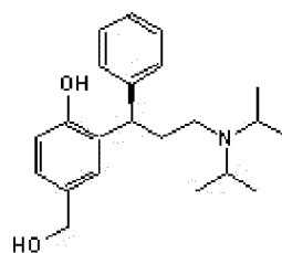
5-hydroxymethyl Tolterodine
