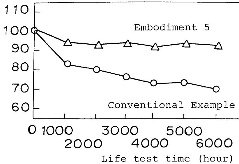
Change of cut-off voltage (%)
