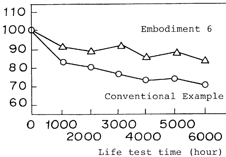
Change of cut-off voltage (%)
