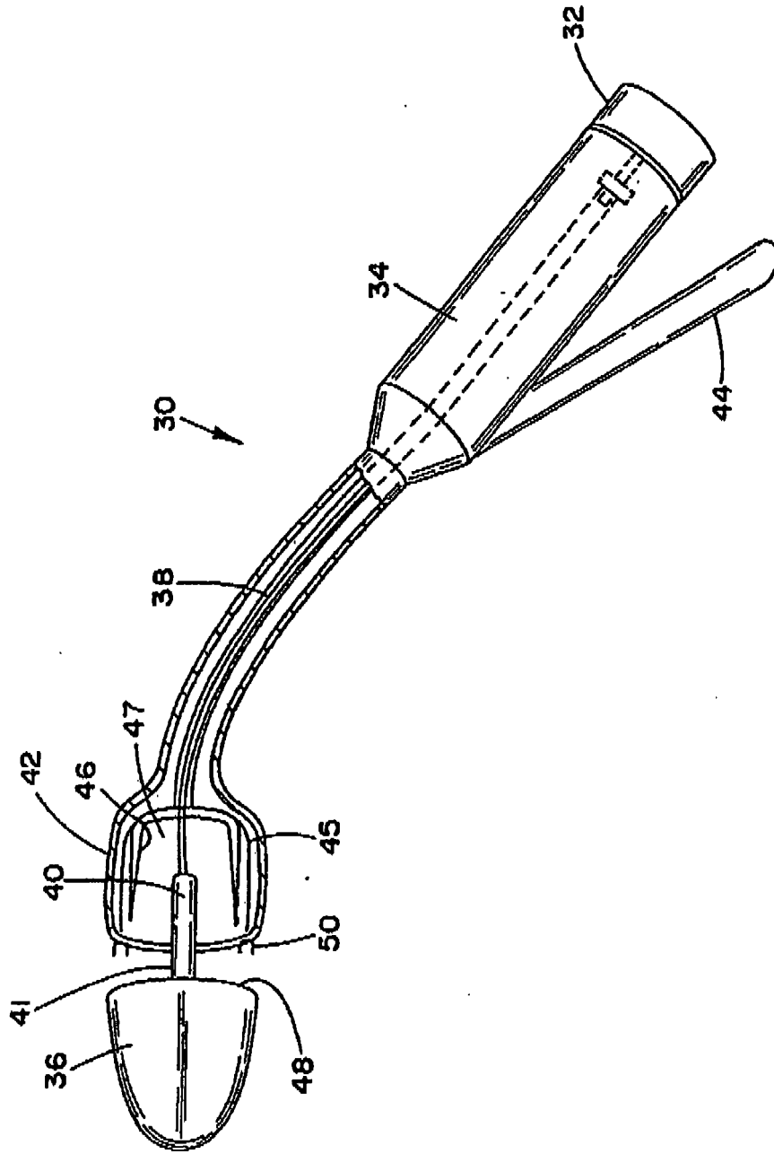
FIG. 2 (PRIOR ART)
