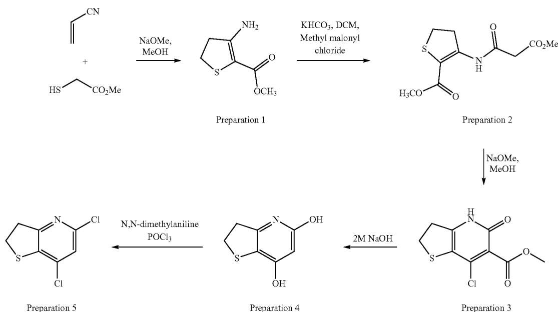
Scheme 1 Synthesis of 5,7-dichloro-2,3-dihydrothieno[3,2-b]pyridine (Preparation 5)
