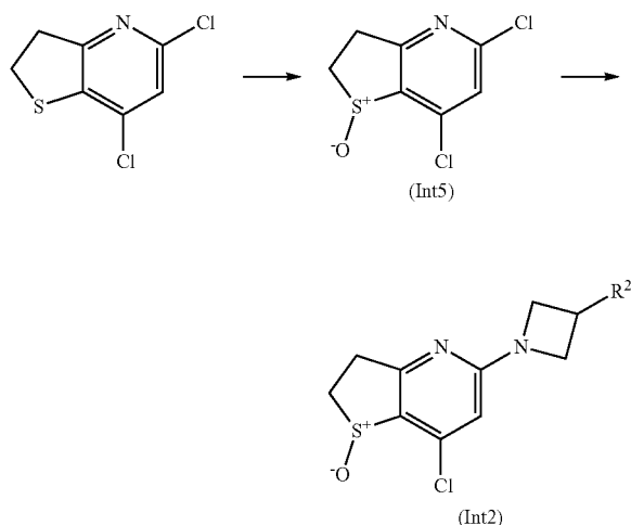
Scheme 3 Alternative synthesis of a compound of general formula (Int2), wherein \text{R}^1 and \text{R}^2 are as previously defined
