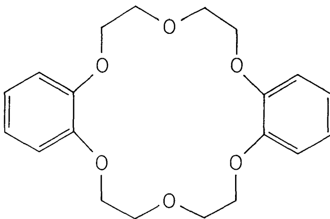
DIBENZOYL-18-CROWN-6
