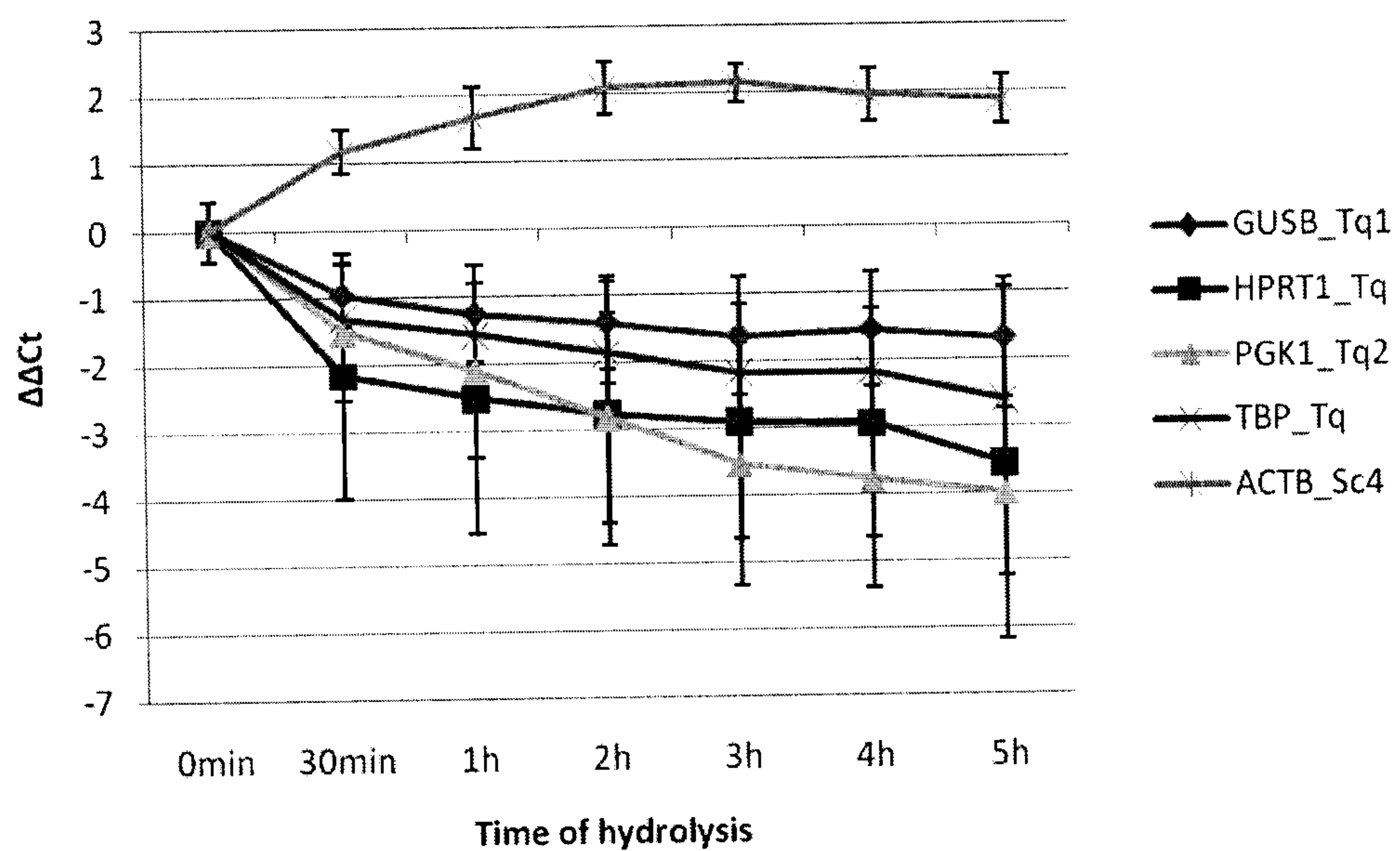
Figure 7. GCC expression variation ( \Delta\Delta C_t ) during NaOH degradation using five reference genes (GUSB, HPRT1, PGK1, TBP and ACTB) for normalization. Variations in delta Ct values ( \Delta\Delta C_t = [(C_{t_{GCC}} - C_{t_{RG}})_{t_x} - (C_{t_{GCC}} - C_{t_{RG}})_{t_0}] ) were determined at each time point of hydrolysis. Error bar represent SD from 3 independent RNA pools. To perform comparison between three experiments, the threshold for each gene was manually fixed to 0.10.
