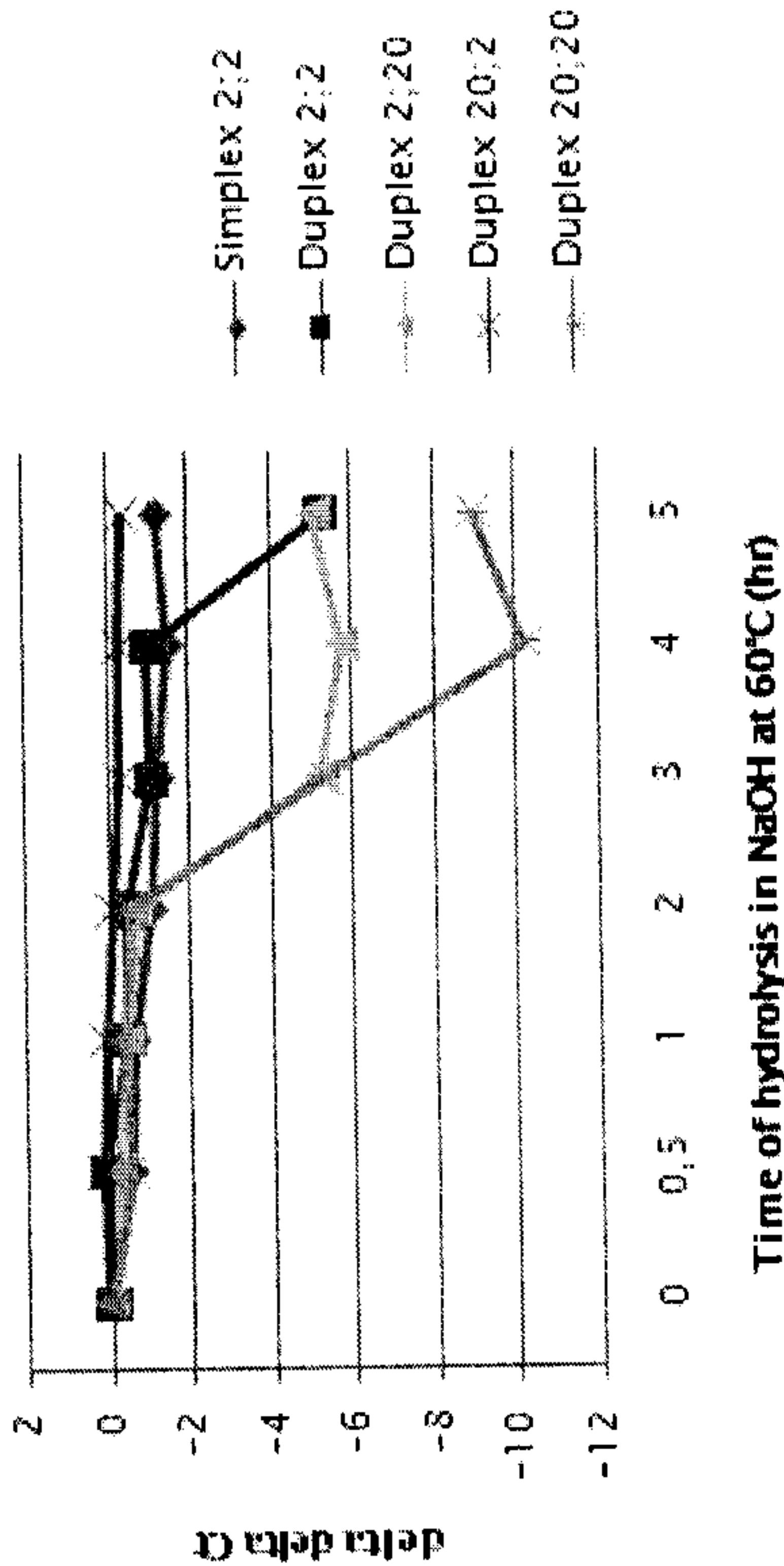
Variation in ΔCt calculation during NaOH degradation
