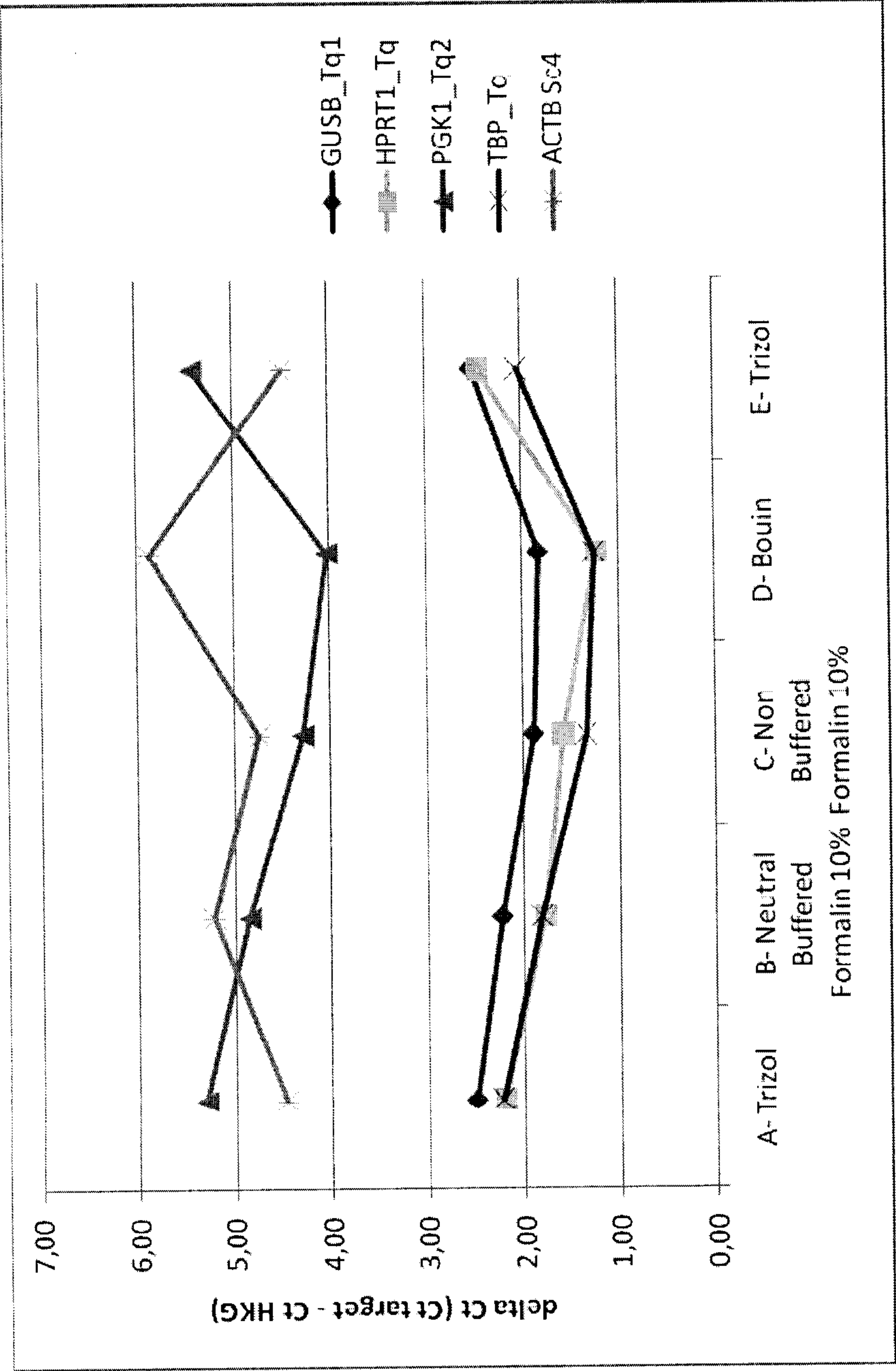
Figure 11. Comparison of GCC expression levels (delta-Ct) in cryo-sections of colon cancer tissue samples fixed or not. Variation in delta Ct values (delta-Ct = (Ct GCC -Ct HKG )) were determined for each RNA extract. The reverse transcription reactions were performed with the SuperScript III First-Strand Synthesis SuperMix (Invitrogen) according to the manufacturer's recommendation, using gene-specific primers (2 µM) and 500 ng of total RNA based on Quant-IT data. The real-time PCR were carried out in a 20-µl reaction volume with the Applied Biosystems 7900HT Fast Real-Time PCR Systems using either TaqMan simplex or the GCC/ACTB duplex assay. Primers and probes concentration for each simplex assays were 900 nM and 250 nM respectively. All reactions were performed in duplicate.
