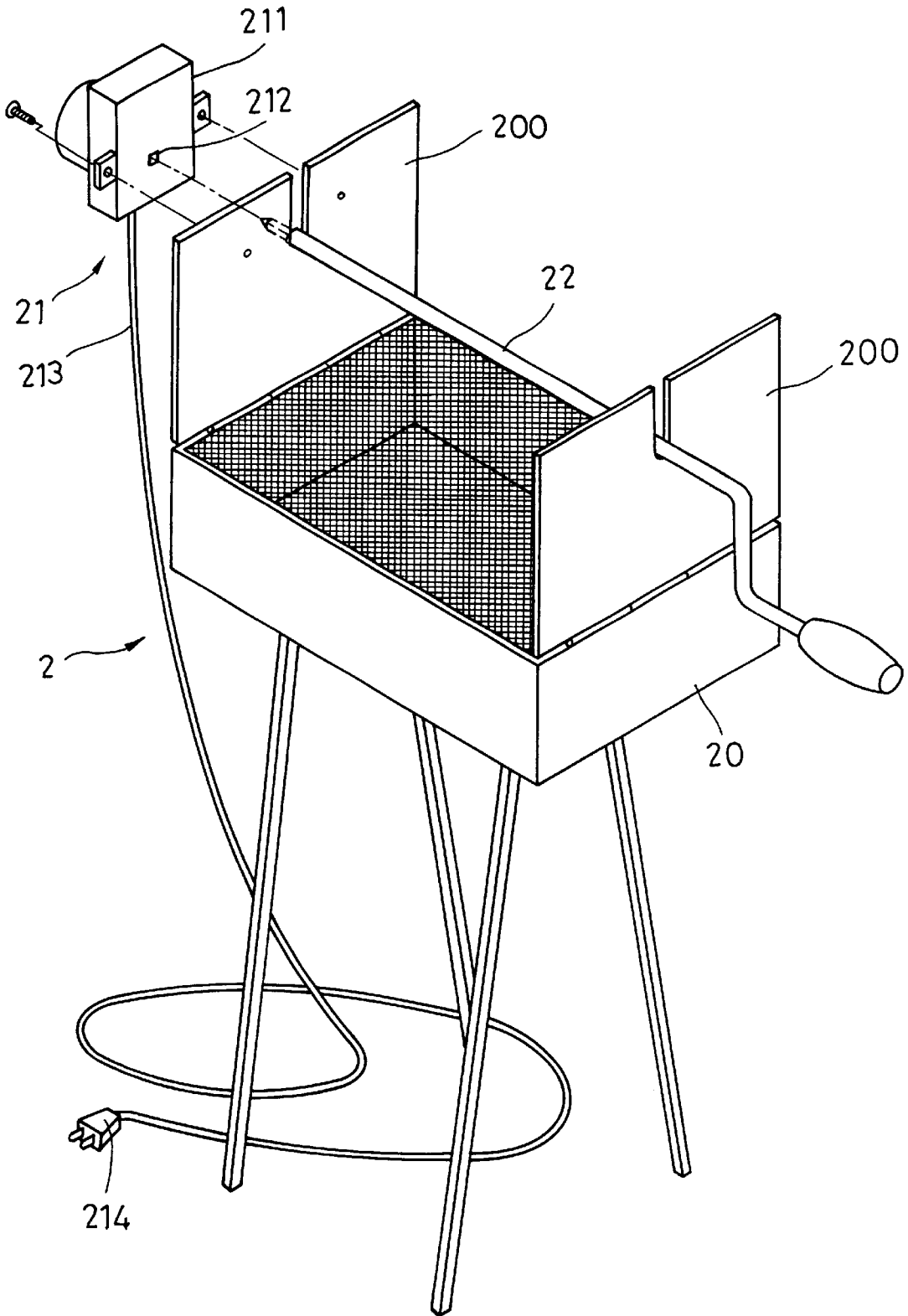
FIG.2 (PRIOR ART)
