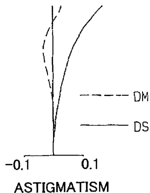
FIG. 14B (W-0.23m) Y'=3.3
