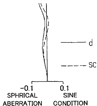
FIG. 16A (T-2.35m) FNO=4.07
