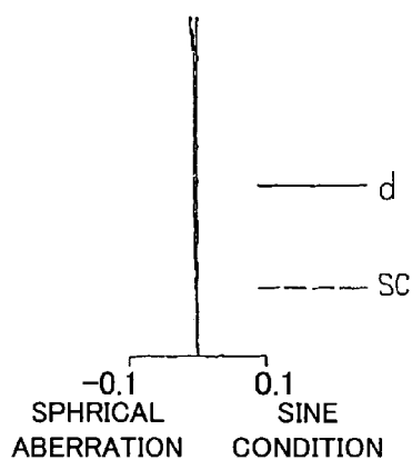
FIG.21A (W-0.15m) FNO=2.91
