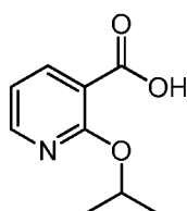
Intermediate H
