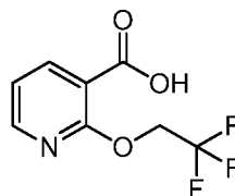
Intermediate J
