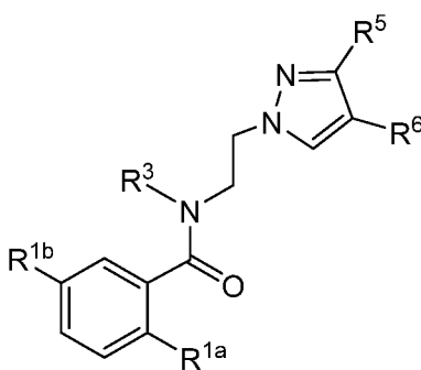
Ic'
