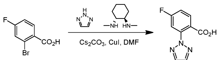
Intermediate F
