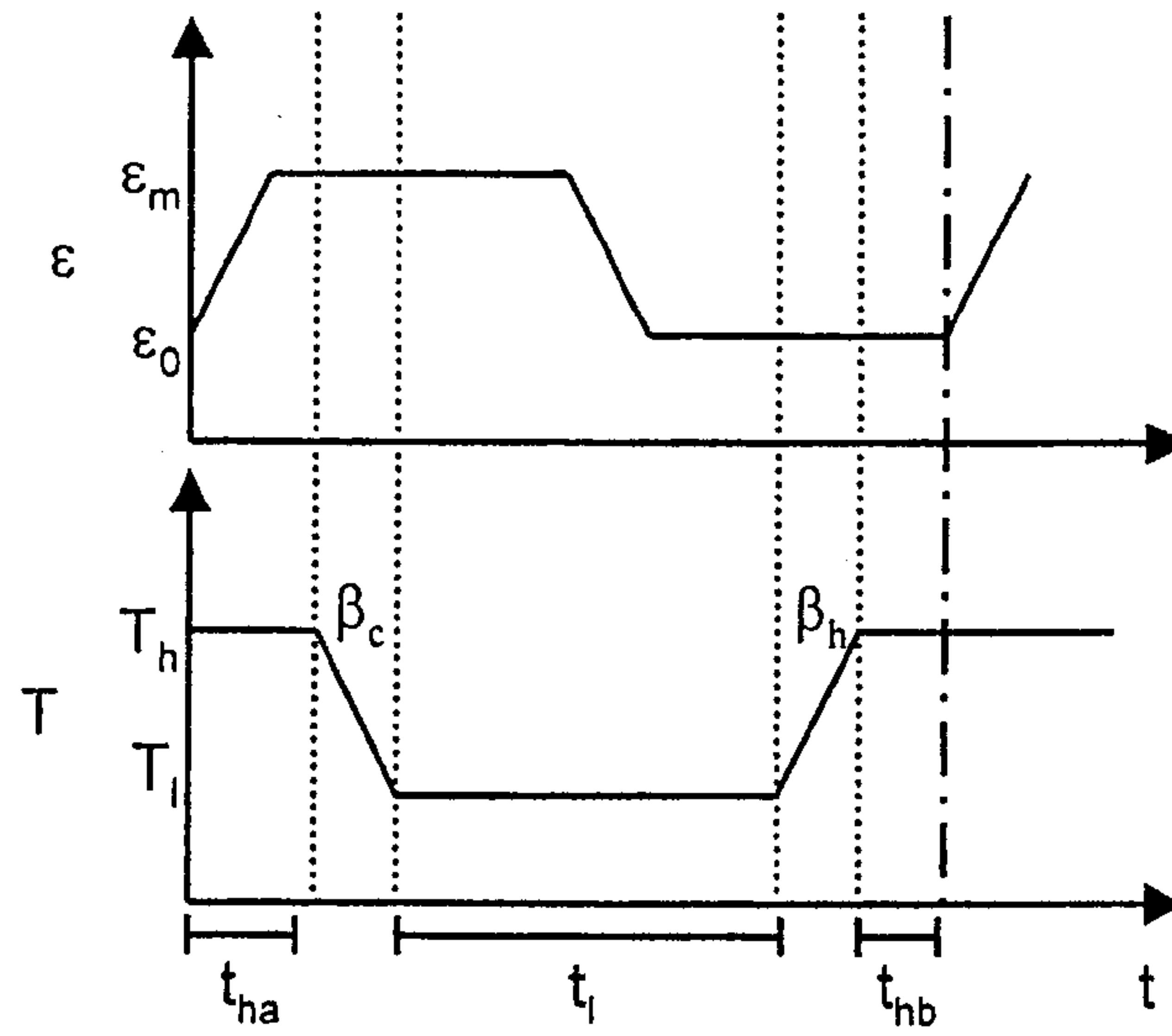
Fig. 2: Schematic representation of the principle of the strain-controlled thermo-mechanical cycle. The change of the temperature from T_h to T_l and from T_l to T_h is indicated with a dotted line (.....). The last vertical line (- - -) identifies the end of the first cycle.
