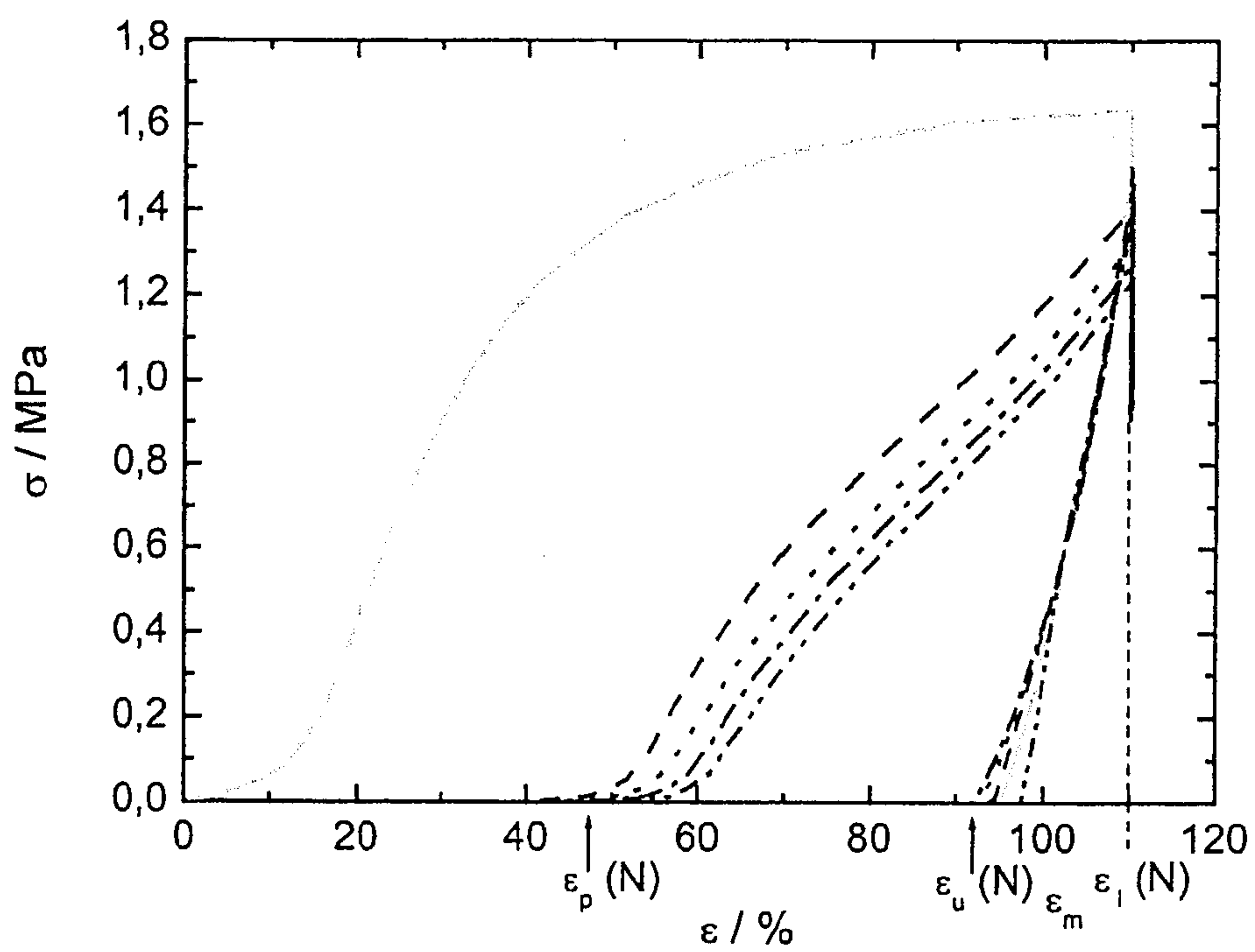
Fig. 3: Illustration of a strain-controlled, cyclical, thermo-mechanical tensile strain experiment with an example of the polymer blend PDA(50) / PCA(47)[22/28] at T_h = 50^\circ\text{C} , T_l = 0^\circ\text{C} and \epsilon_m = 100\% .
