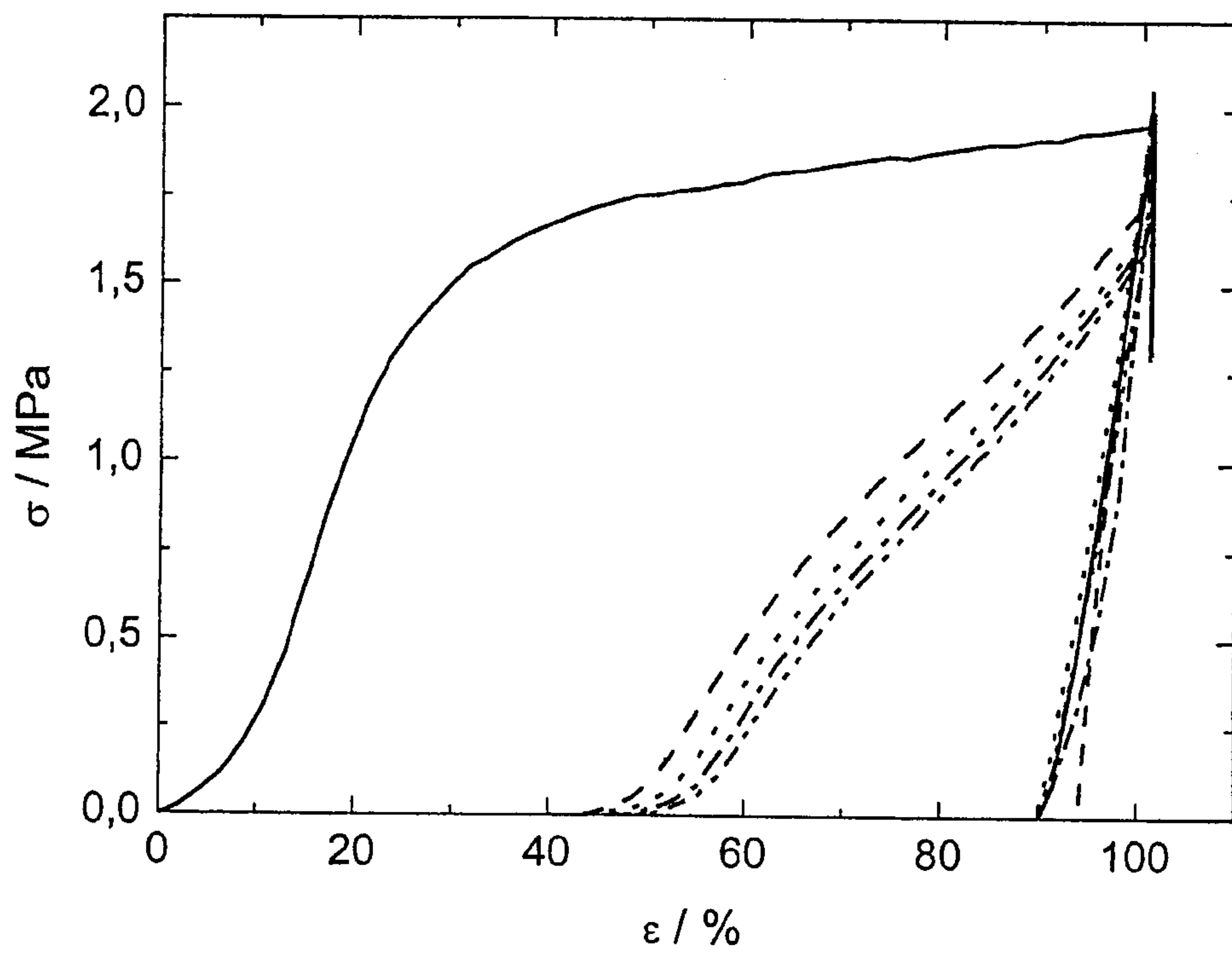
Fig. 6: Illustration of a strain-controlled, cyclical, thermo-mechanical tensile strain experiment with an example of the extruded polymer blend PDA(50) / PCA(68)[30/27] at T_h = 50^\circ\text{C} , T_l = 0^\circ\text{C} and \varepsilon_m = 100\% .
