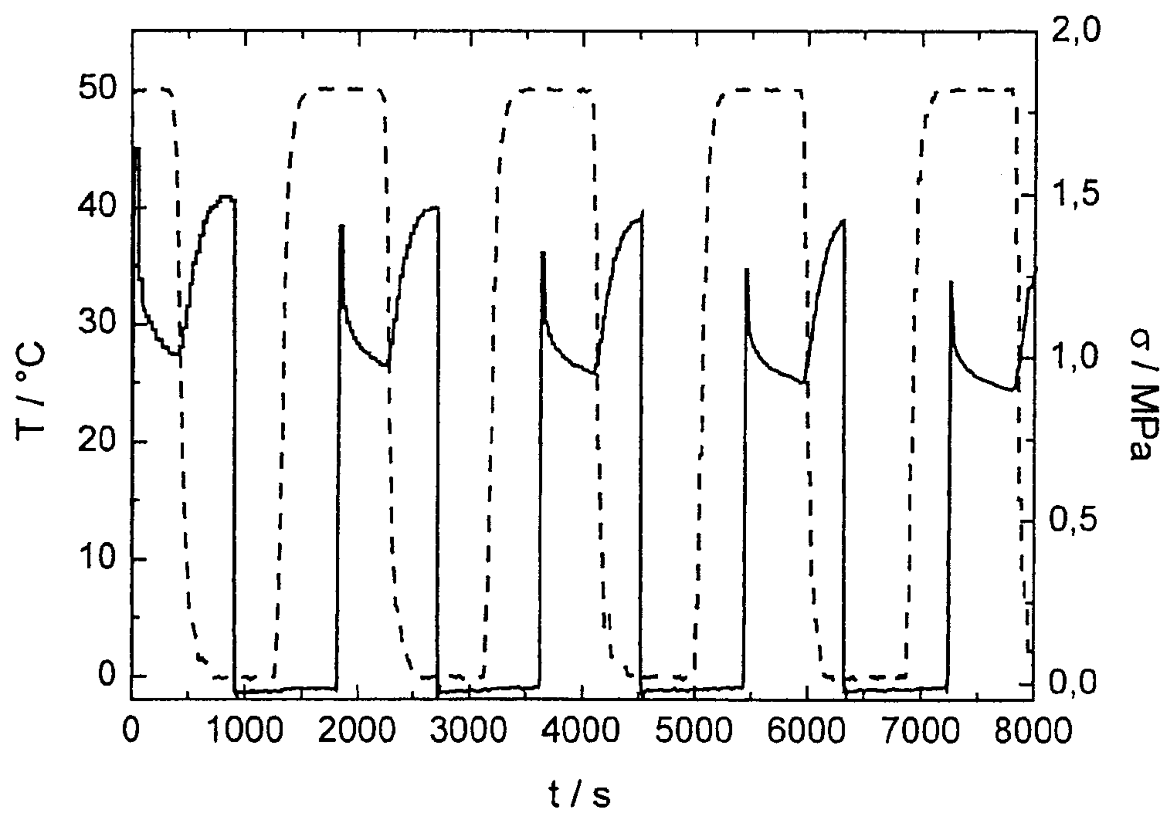
Fig. 4: Temperature T (---) and stress \sigma (-) in dependence of time during a strain-controlled, cyclical, thermo-mechanical cycle for an example of the polymer blend PDA(50) / PCA(47)[22/28].
