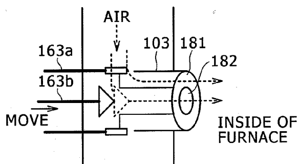
FIG. 11D AFTER-AIR PORT
