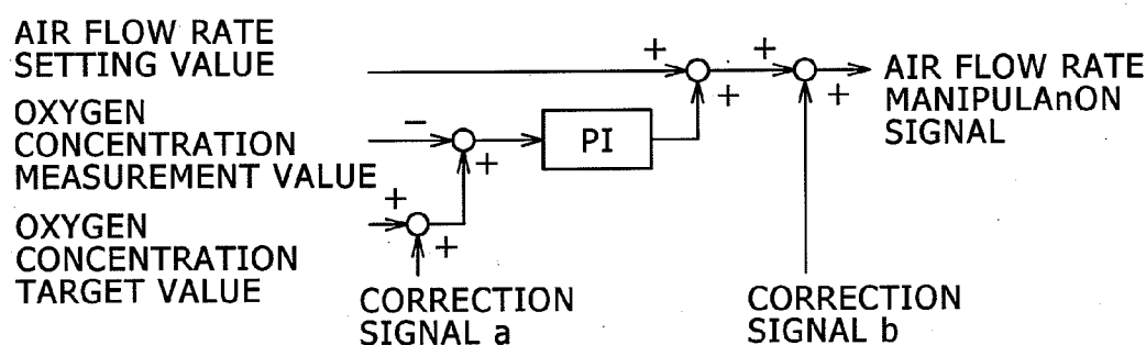
FIG. 11C MANIPULATION SIGNAL CORRECTION
