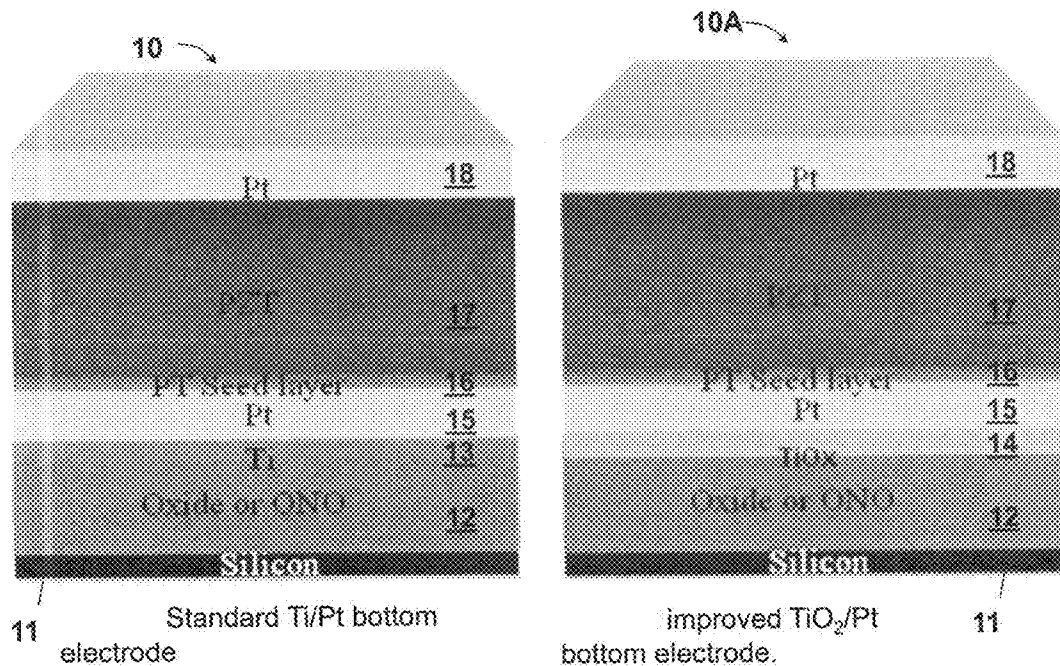
Wafer stacks showing the different layers
