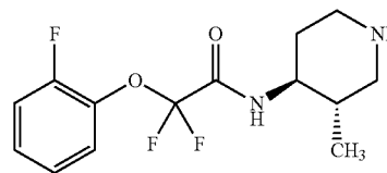
Example 54: 2,2-difluoro-2-(2-fluorophenoxy)-N-((3S,4S)-3-methylpiperidin-4-yl)acetamide
