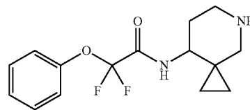
Example 49: 2,2-difluoro-2-phenoxy-N-(5-azaspiro[2.5]octan-8-yl)acetamide
