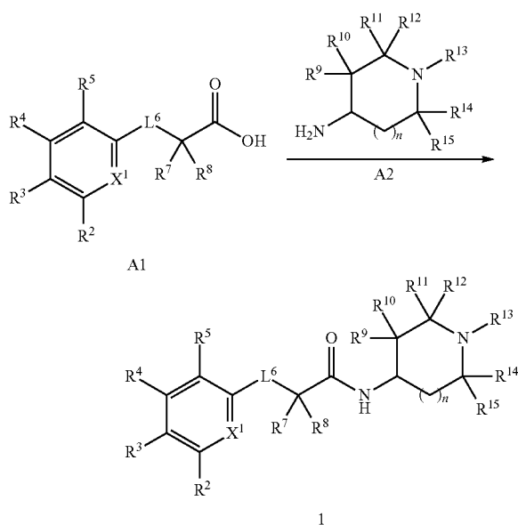
Scheme A
