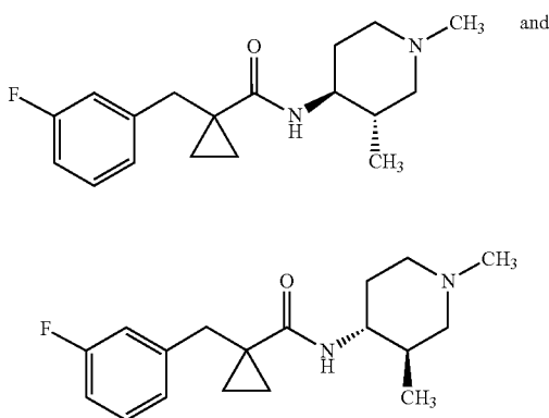
Example 20: N-(trans-1,3-dimethylpiperidin-4-yl)-1-(3-fluorobenzyl)cyclopropane-1-carboxamide
