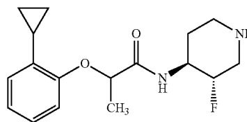
Example 63: 2-(2-cyclopropylphenoxy)-N-((3S,4S)-3-fluoropiperidin-4-yl)propanamide
