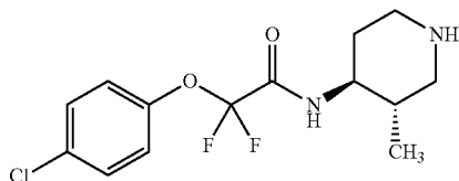
Example 66: 2-(4-chlorophenoxy)-2,2-difluoro-N-((3S,4S)-3-methylpiperidin-4-yl)acetamide
