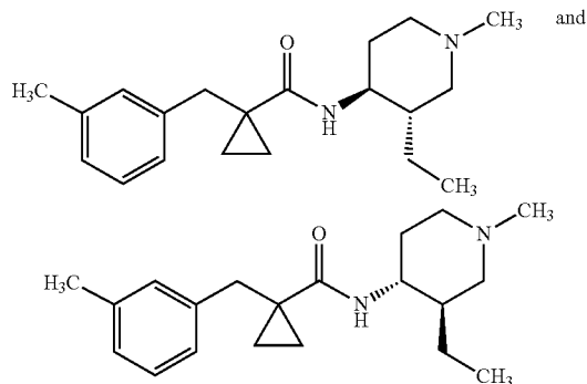
Example 21: N-(trans-3-ethyl-1-methylpiperidin-4-yl)-1-(3-methylbenzyl)cyclopropane-1-carboxamide
