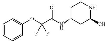
Example 53: 2,2-difluoro-N-((2S,4R)-2-methylpiperidin-4-yl)-2-phenoxyacetamide
