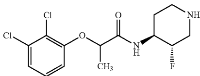
Example 61: 2-(2,3-dichlorophenoxy)-N-((3S,4S)-3-fluoropiperidin-4-yl)propanamide
