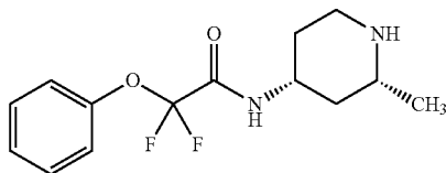
Example 51: 2,2-difluoro-N-((2R,4R)-2-methylpiperidin-4-yl)-2-phenoxyacetamide
