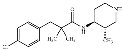
Example 19: 3-(4-chlorophenyl)-2,2-dimethyl-N-((3S,4S)-3-methylpiperidin-4-yl)propanamide
