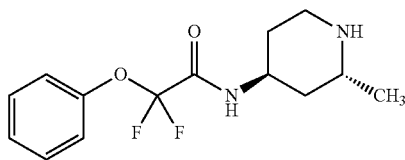
Example 52: 2,2-difluoro-N-((2R,4S)-2-methylpiperidin-4-yl)-2-phenoxyacetamide
