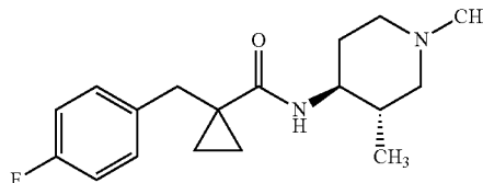
Example 35: N-((3S,4S)-1,3-dimethylpiperidin-4-yl)-1-(4-fluorobenzyl)cyclopropane-1-carboxamide
