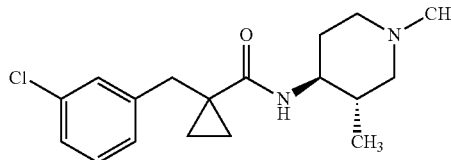
Example 36: 1-(3-chlorobenzyl)-N-((3S,4S)-1,3-dimethylpiperidin-4-yl)cyclopropane-1-carboxamide
