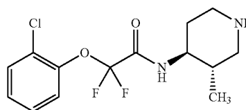
Example 64: 2-(2-chlorophenoxy)-2,2-difluoro-N-((3S,4S)-3-methylpiperidin-4-yl)acetamide
