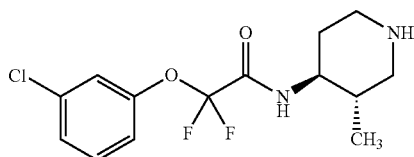
Example 65: 2-(3-chlorophenoxy)-2,2-difluoro-N-((3S,4S)-3-methylpiperidin-4-yl)acetamide
