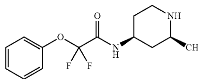
Example 48: 2,2-difluoro-N-((2S,4S)-2-methylpiperidin-4-yl)-2-phenoxyacetamide
