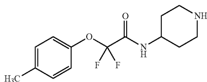
Example 34: 2,2-difluoro-N-(piperidin-4-yl)-2-(p-tolyloxy)acetamide
