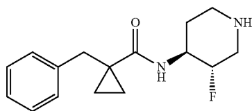
Example 45: 1-benzyl-N-((3S,4S)-3-fluoropiperidin-4-yl)cyclopropane-1-carboxamide
