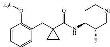
Example 47: N-((3S,4S)-3-fluoropiperidin-4-yl)-1-(2-methoxybenzyl)cyclopropane-1-carboxamide
