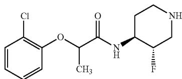
Example 62: 2-(2-chlorophenoxy)-N-((3S,4S)-3-fluoropiperidin-4-yl)propanamide
