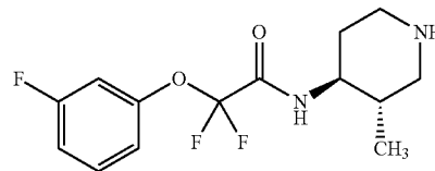
Example 55: 2,2-difluoro-2-(3-fluorophenoxy)-N-((3S,4S)-3-methylpiperidin-4-yl)acetamide
