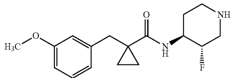
Example 46: N-((3S,4S)-3-fluoropiperidin-4-yl)-1-(3-methoxybenzyl)cyclopropane-1-carboxamide
