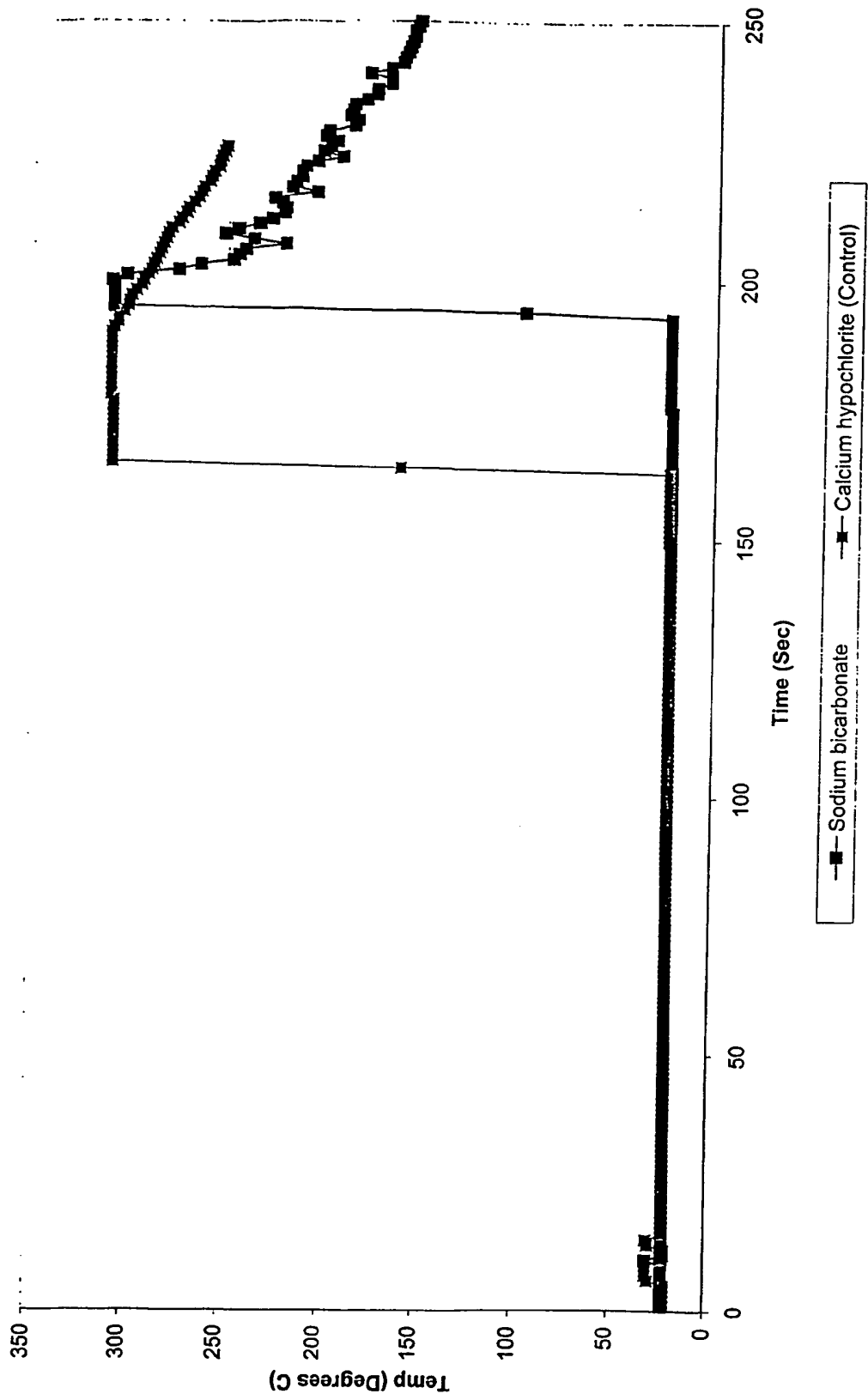
Figure 3 Calcium Hypochlorite + Brake Fluid Compared to a Blend of Calcium Hypochlorite and Sodium Bicarbonate + Brake Fluid
