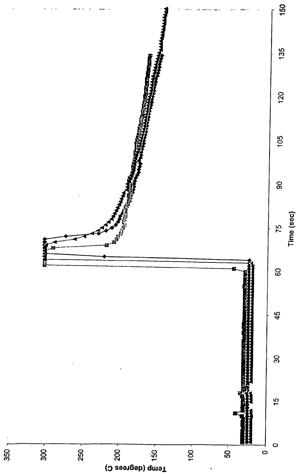
Figure 1 3 Replicate Calcium Hypochlorite + Brake Fluid Reactions
