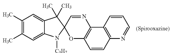
Photochromic compound II:
