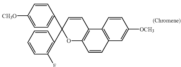
Photochromic compound II:
