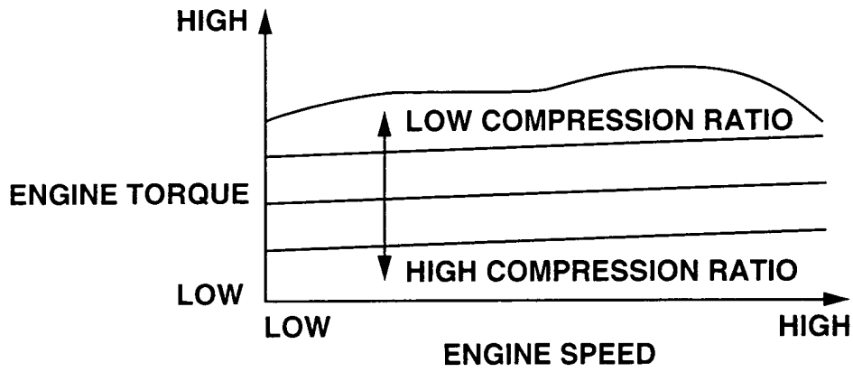
COMPRESSION RATIO MAP
