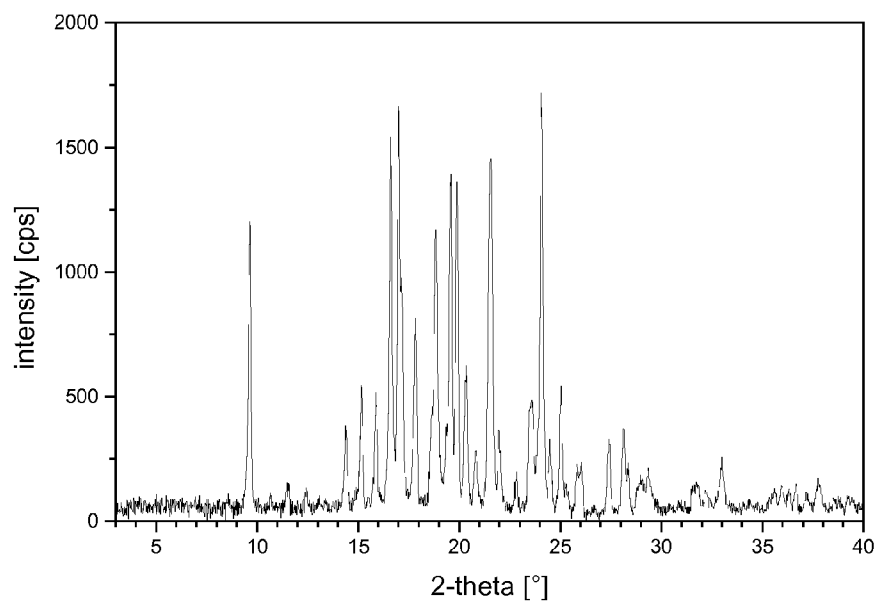
Figure 1.21: X-ray powder diffraction diagram of Fum 3 = fumarate, form III
