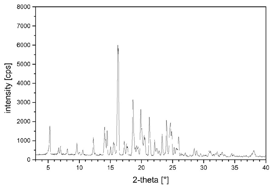
Figure 1.23: X-ray powder diffraction diagram of Cas 2 = camphorsulfonate, form II
