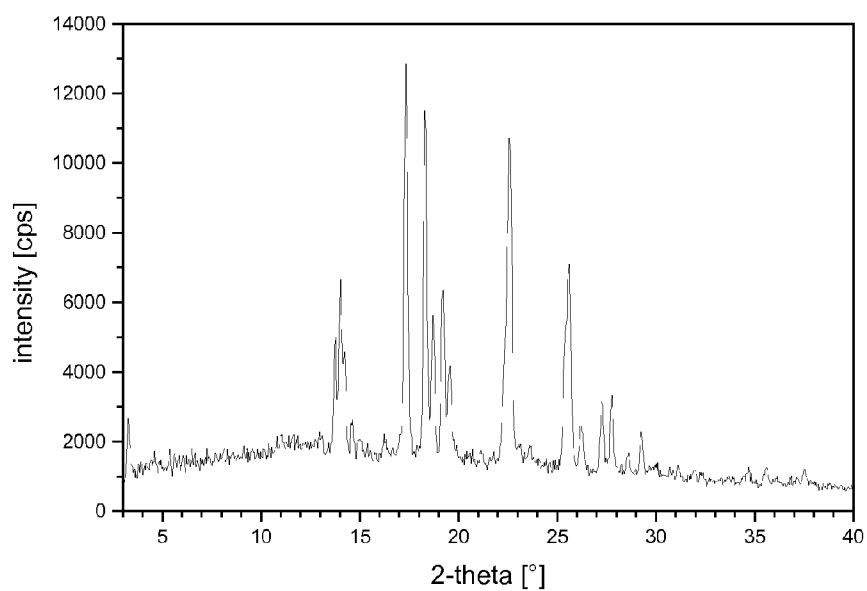
Figure 1.4 X-ray powder diffraction diagram of Tos1 = tosylate, form I
