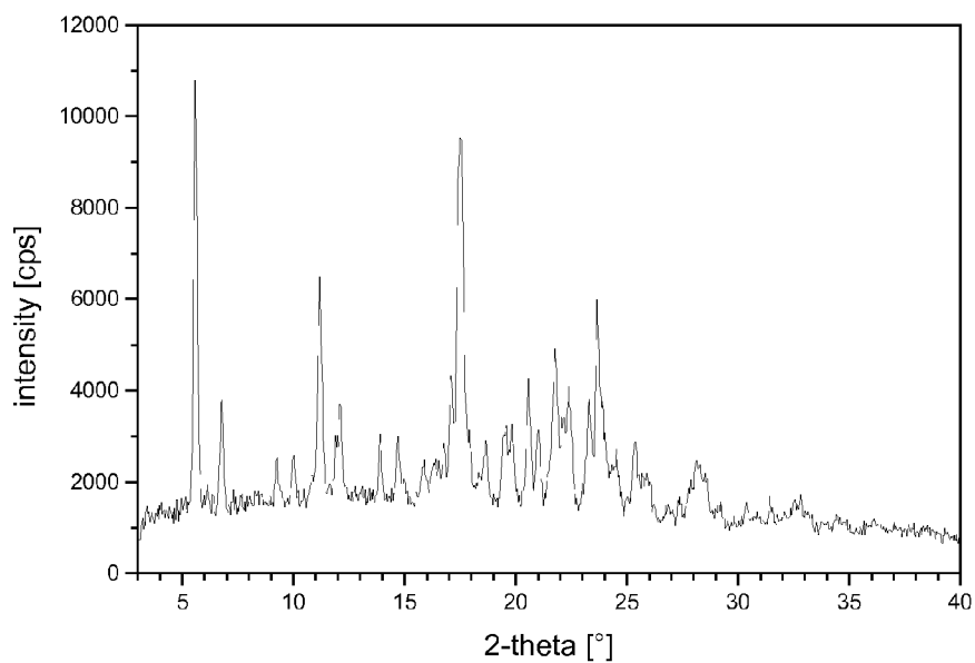
Figure 1.9 X-ray powder diffraction diagram of Pho1 = phosphate, form I
