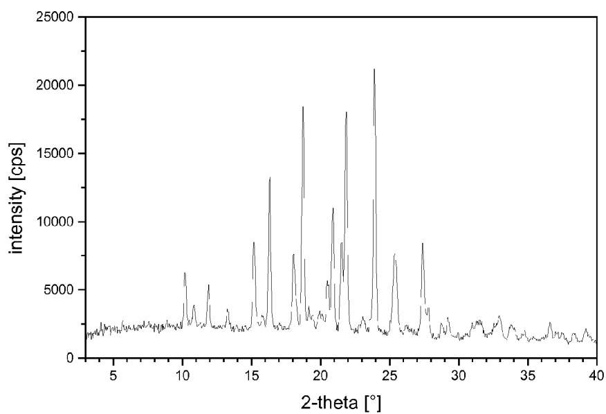
Figure 1.15b: X-ray powder diffraction diagram of Fum 2 = fumarate, form II
