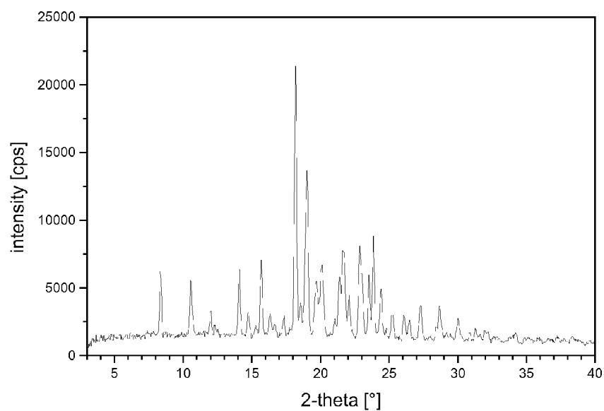
Figure 1.18: X-ray powder diffraction diagram of Man 1 = mandelate, form I
