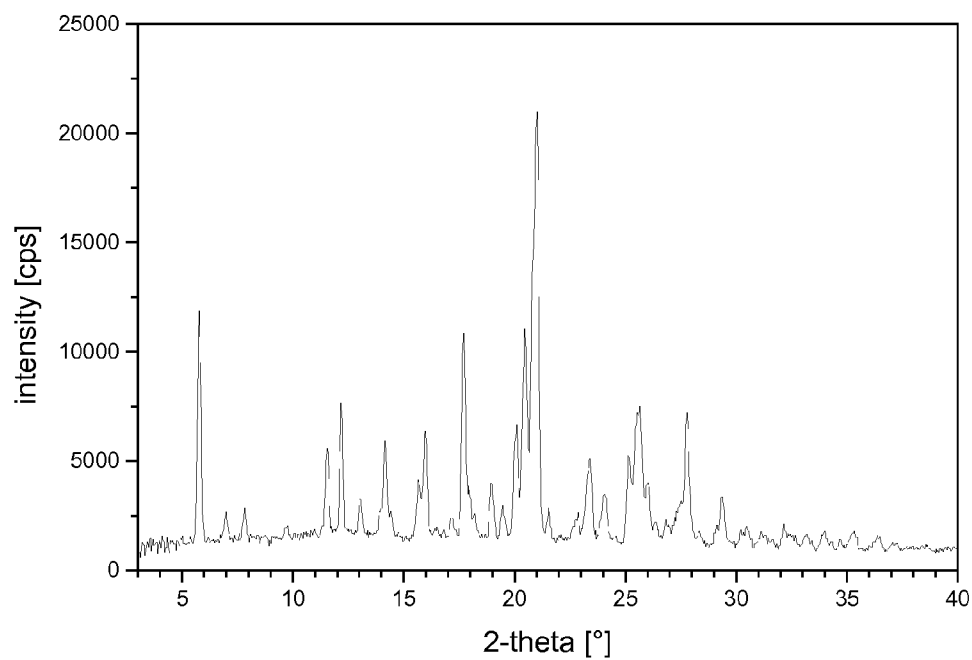
Figure 1.11: X-ray powder diffraction diagram of Ets 1 = ethanesulfonate, form I
