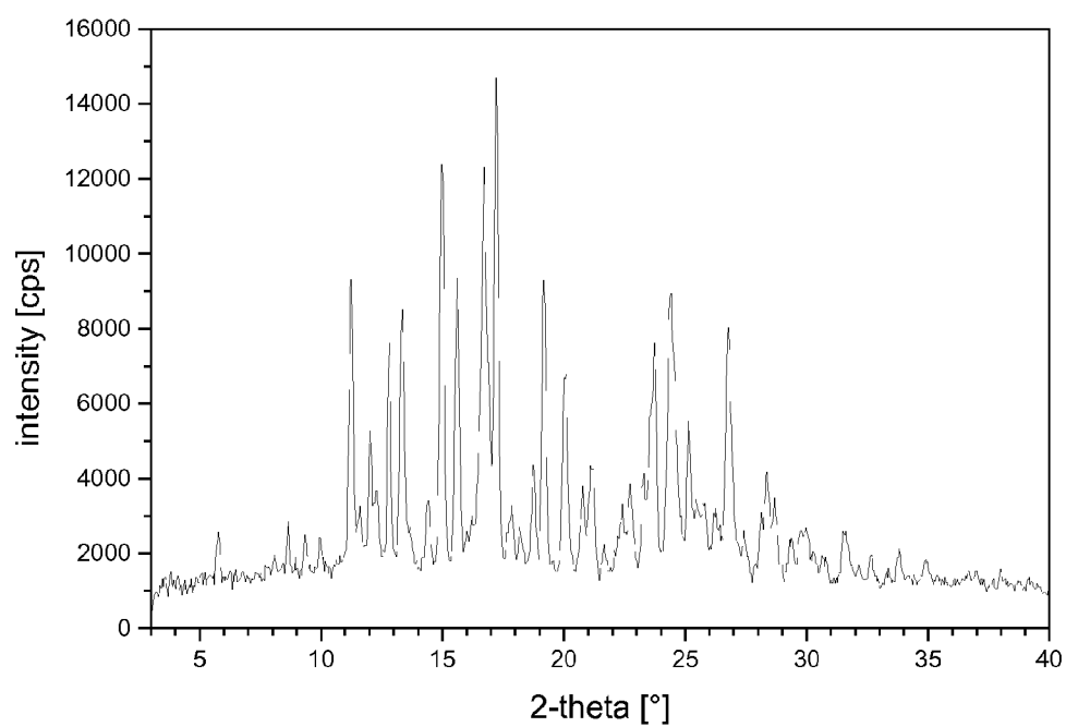
Figure 1.8 X-ray powder diffraction diagram of Sac 1 = sacharinate, form I
