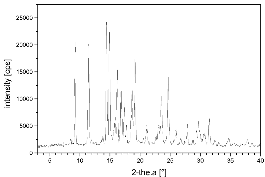
Figure 1.10b: X-ray powder diffraction diagram of Mae 3 = maleate, form III
