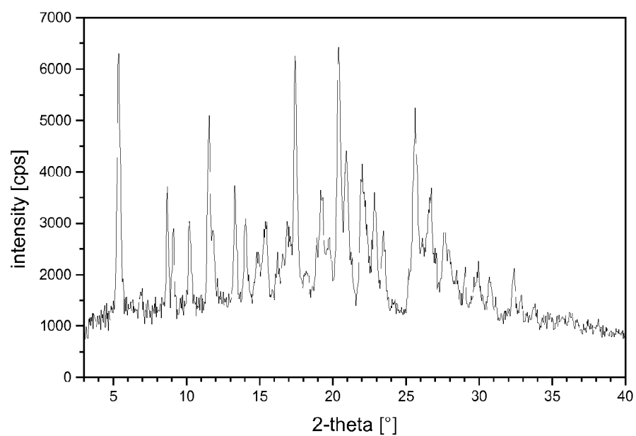
Figure 1.1b X-ray powder diffraction diagram of HCl3 = chloride, form III
