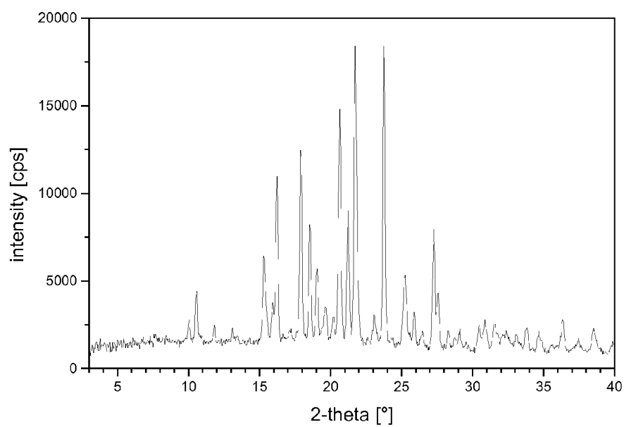
Figure 1.14: X-ray powder diffraction diagram of L-Tar 1 = L-tartrate, form I
