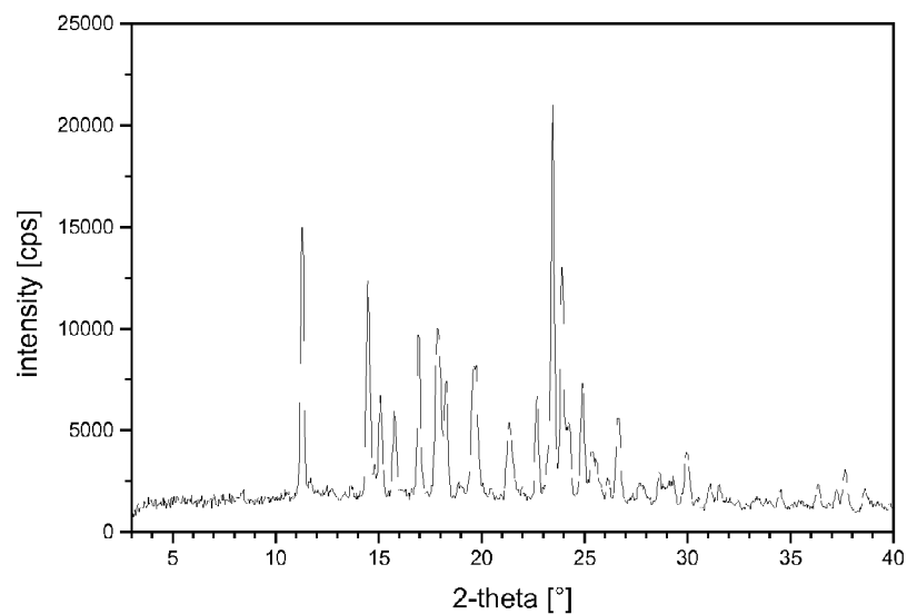
Figure 1.19: X-ray powder diffraction diagram of L-Mal 1 = L-malate, form I
