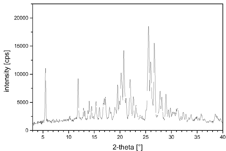
Figure 1.2b X-ray powder diffraction diagram of HBr3 = hydrobromid, form III
