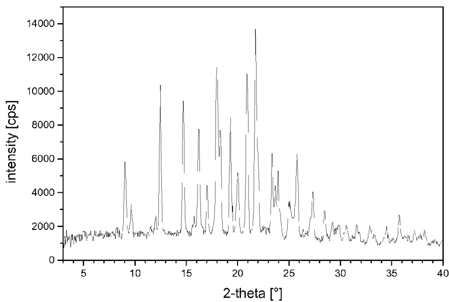
Figure 1.7b X-ray powder diffraction diagram of Oxa 5 = oxalate, form V
