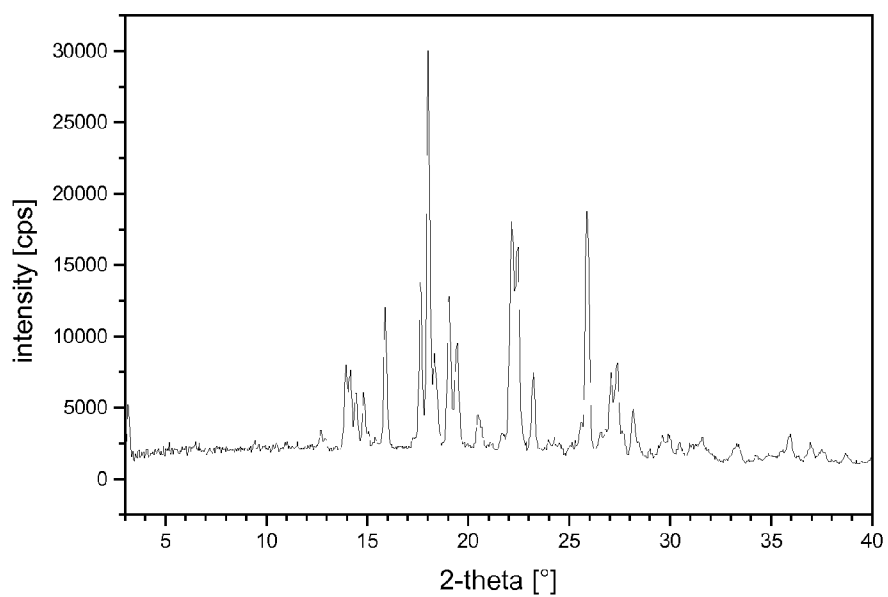
Figure 1.21: X-ray powder diffraction diagram of Fum 3 = fumarate, form III
