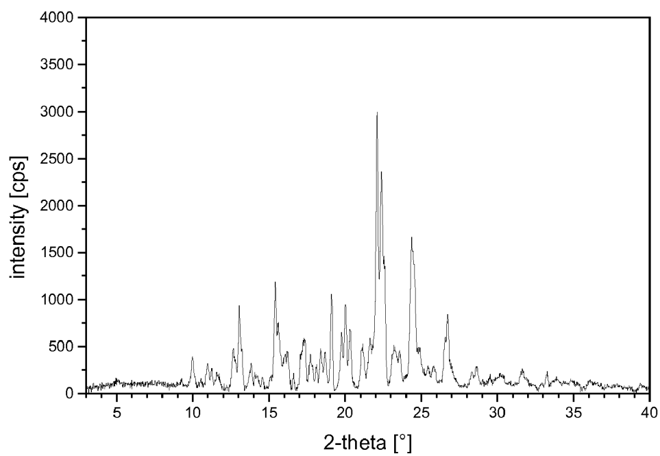
Figure 1.24: X-ray powder diffraction diagram of Gly 3 = glycolate, form II
