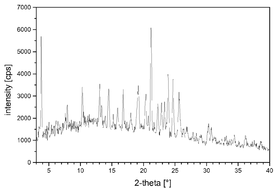
Figure 1.13: X-ray powder diffraction diagram of Mao 1 = malonate, form I
