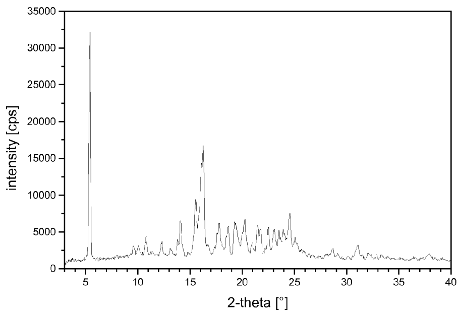
Figure 1.12 X-ray powder diffraction diagram of Cas1 = camphorsulfonate, form I
