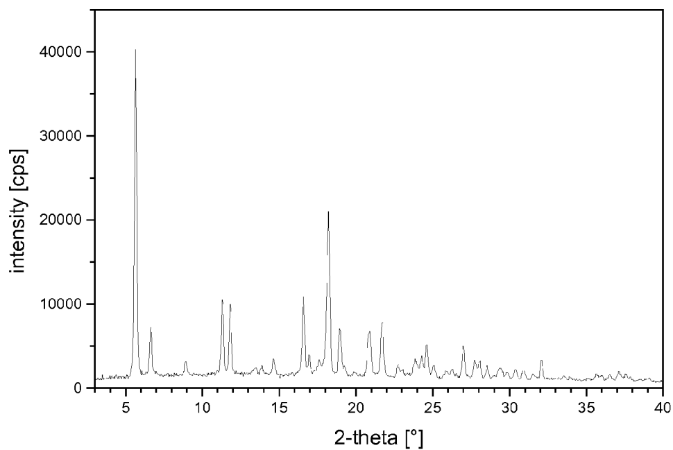
Figure 1.17: X-ray powder diffraction diagram of Cit 1 = citrate, form I
