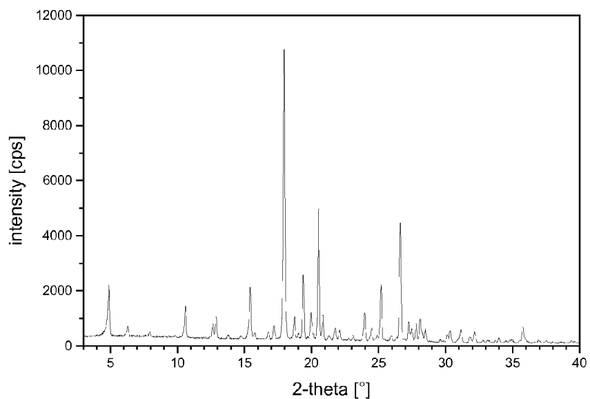
Figure 1.23: X-ray powder diffraction diagram of Cas 2 = camphorsulfonate, form II
