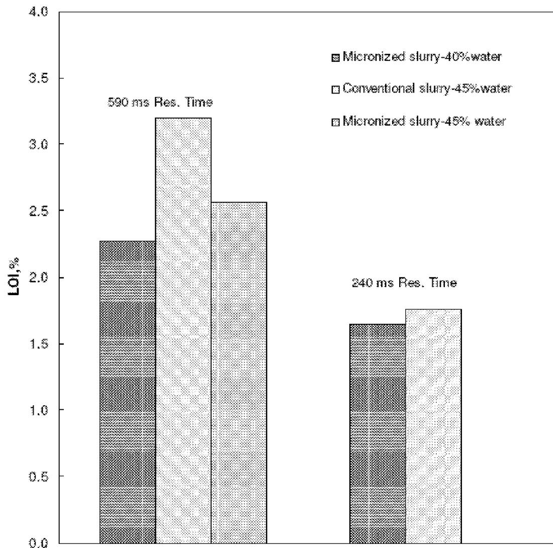
Comparison of Loss on Ignition (LOI).
