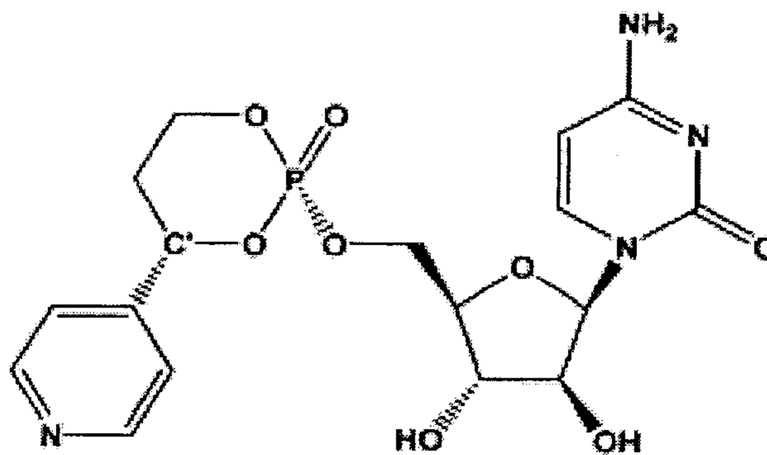
Formula III
