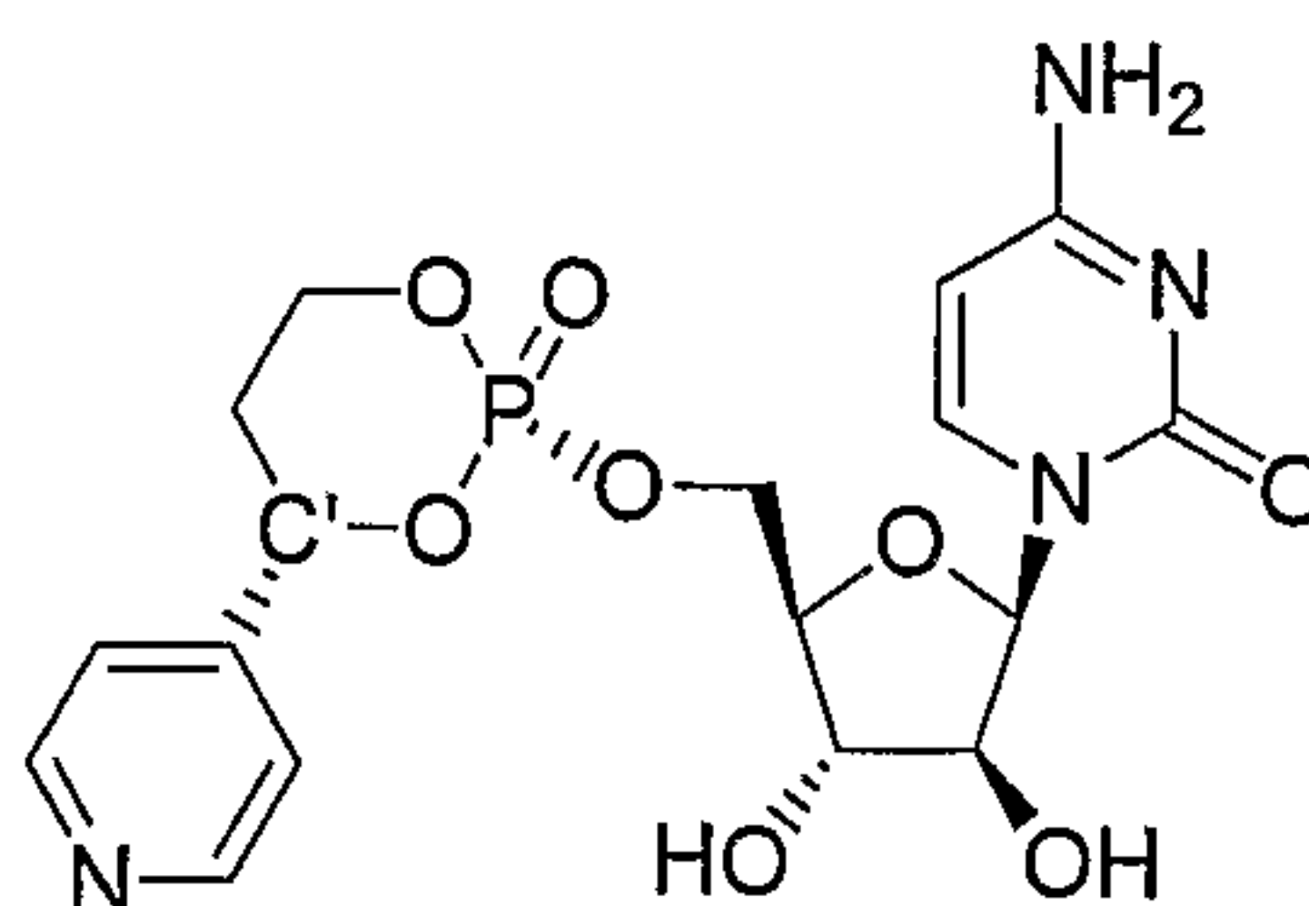
Formula III
