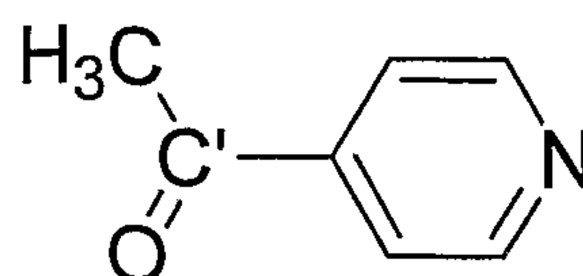
Formula A
