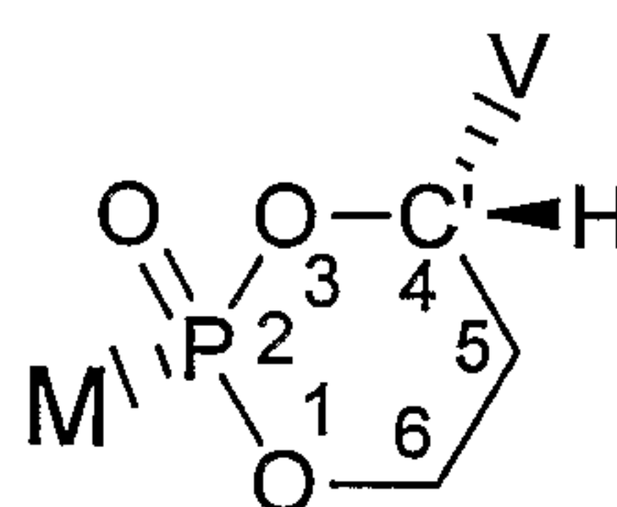
Formula II
