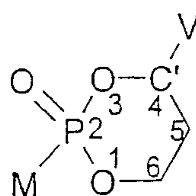
Formula I
