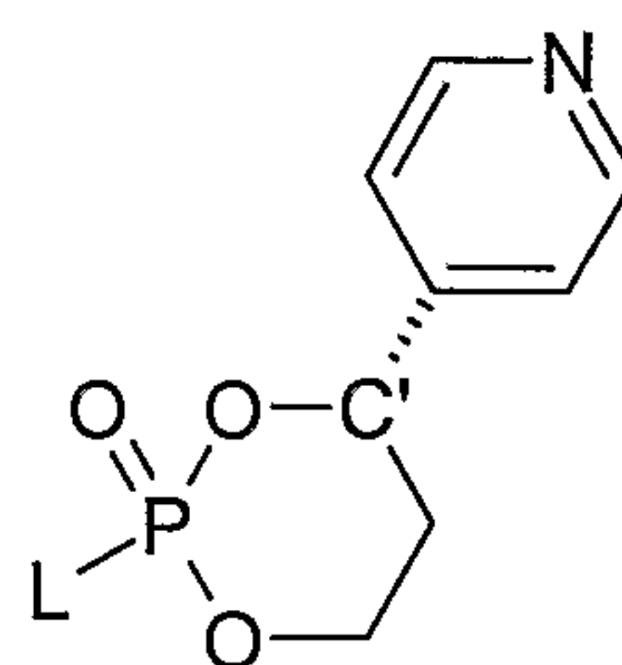
Formula IV
