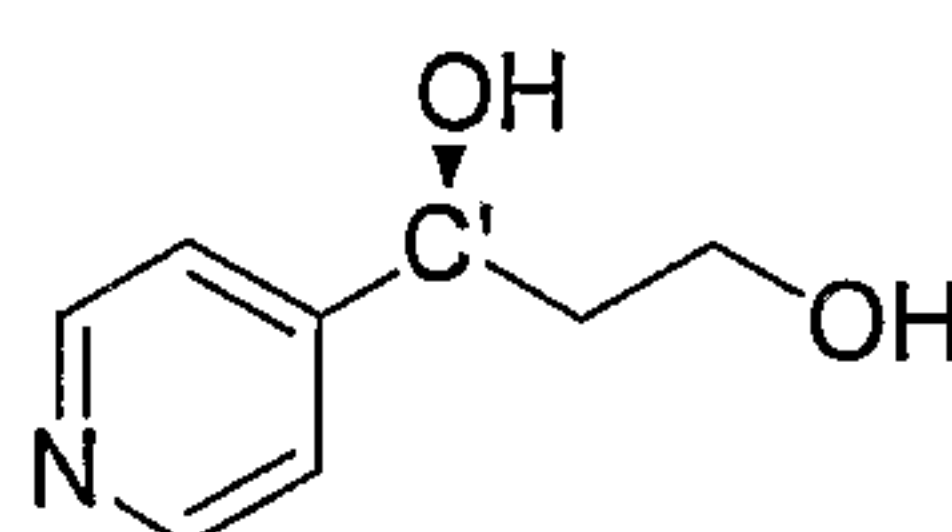
Formula B
