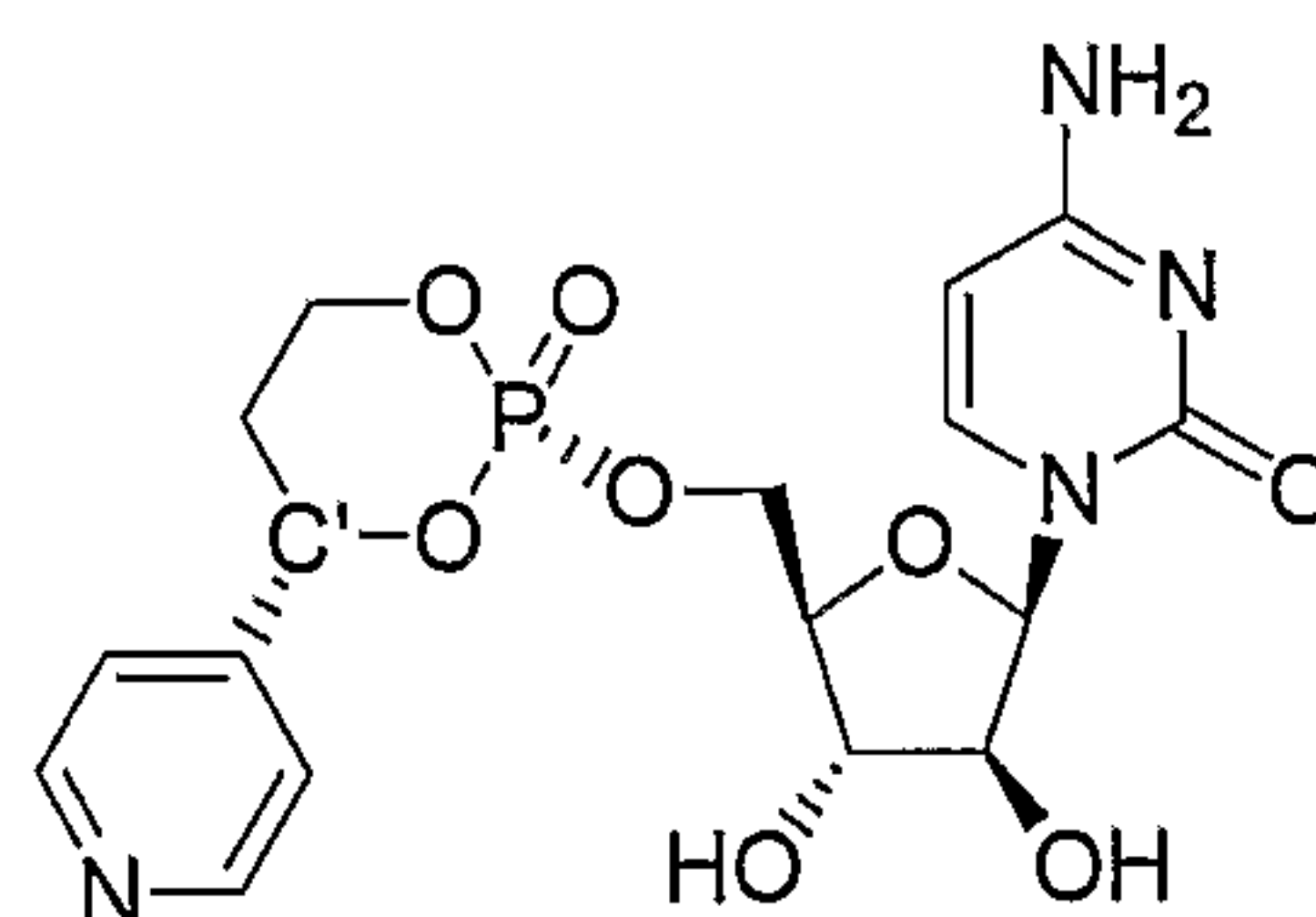
Formula III
