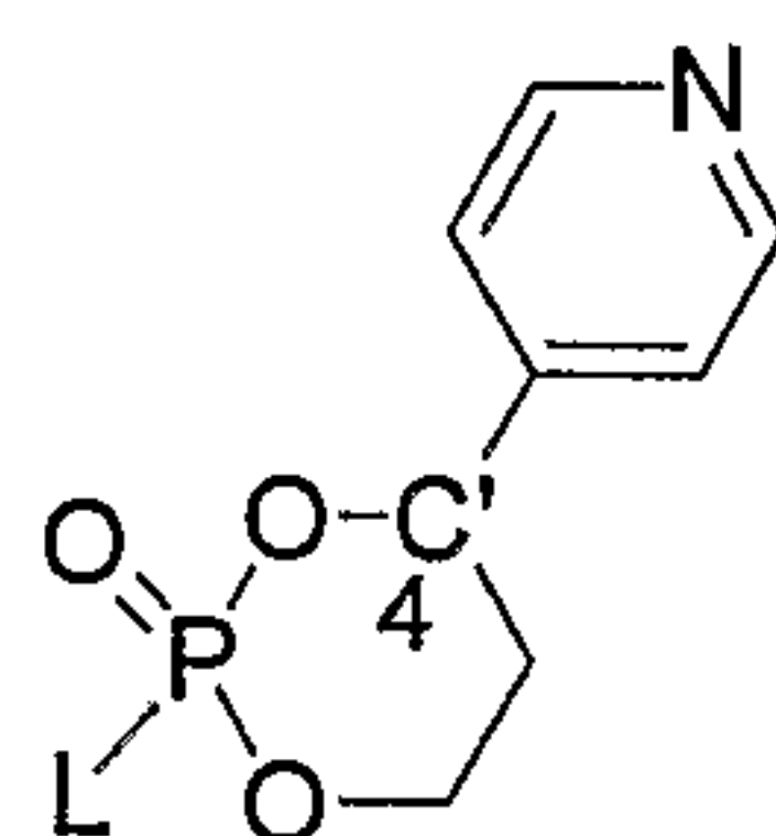
Formula C
