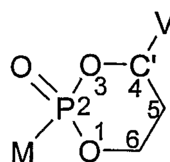
Formula I
