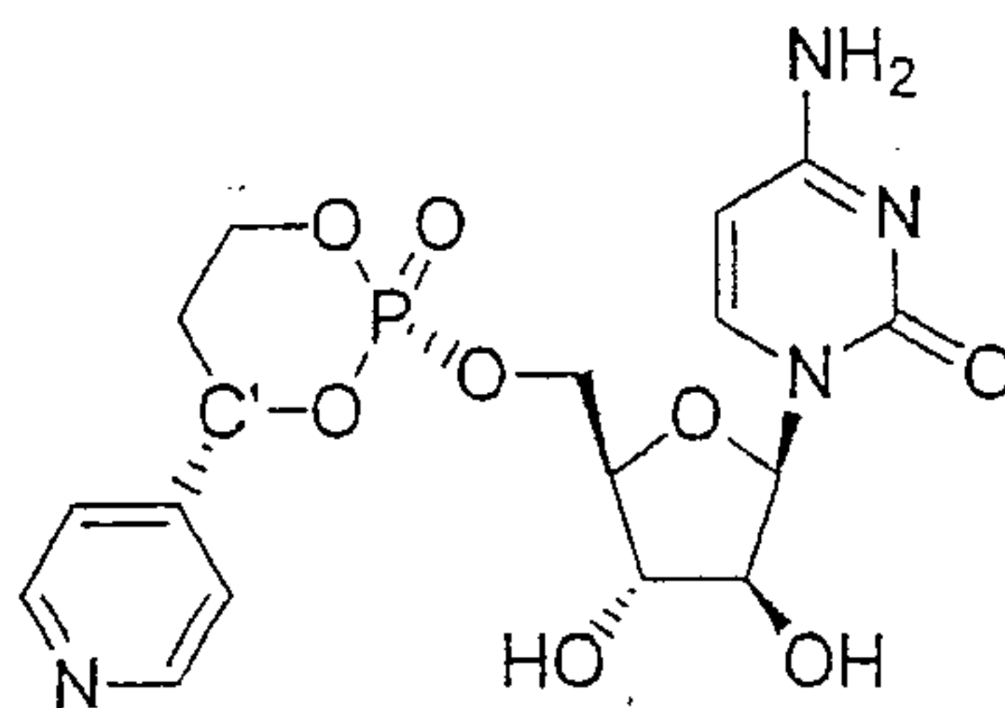
Formula III
