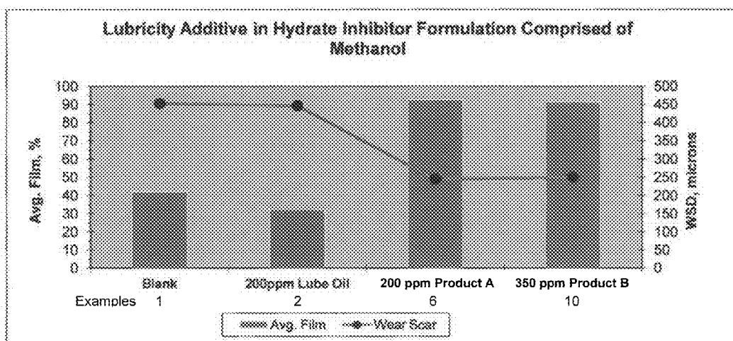
Products A and B Lubricity Performance Graph
