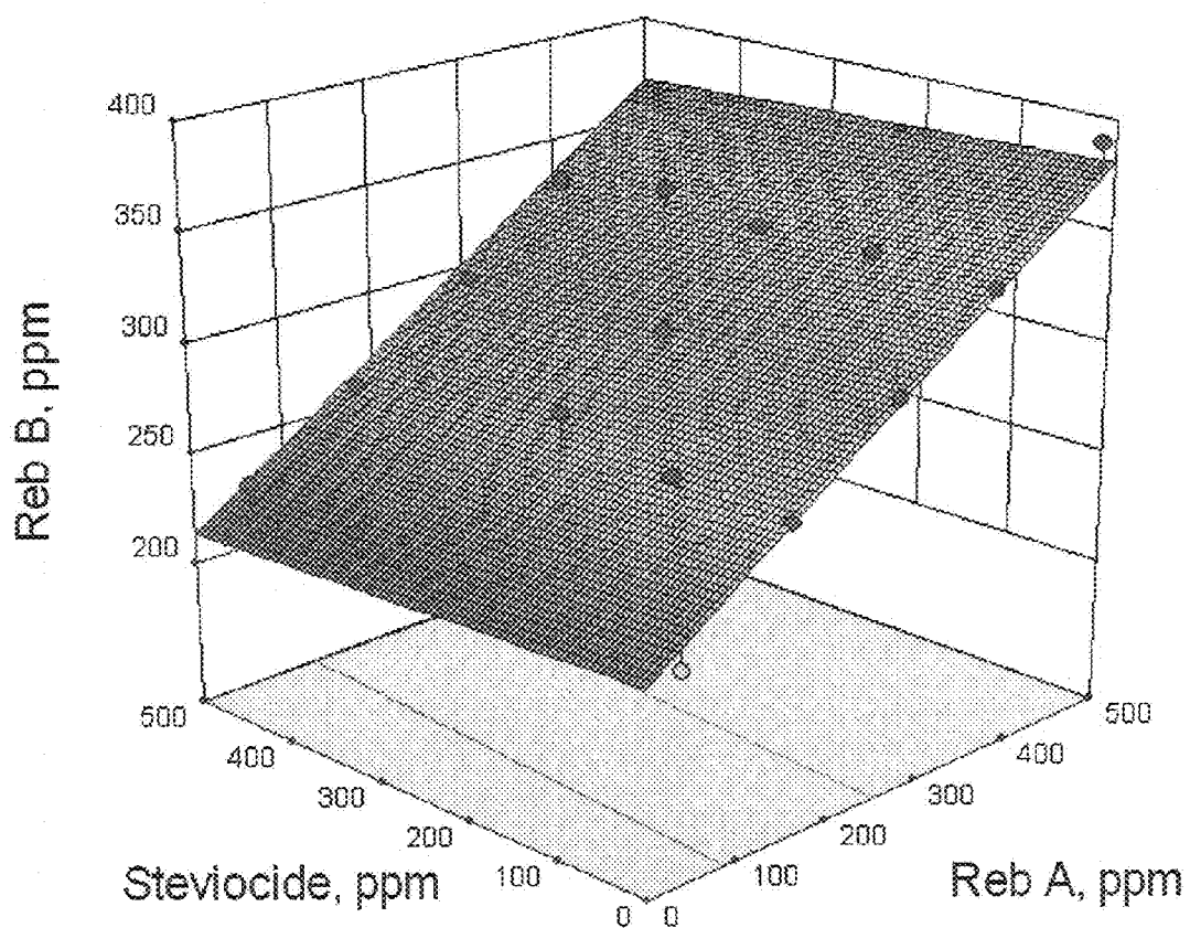
Figure 1 The solubility of Reb B, as a function of Reb A and Steviocide concentrations, in pH 3 citric acid/citrate buffer
