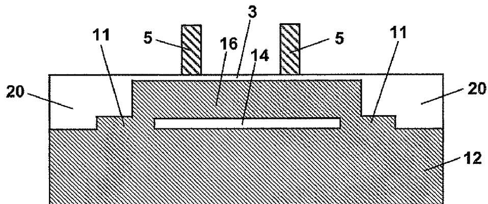
Figure 1C (PRIOR ART)
