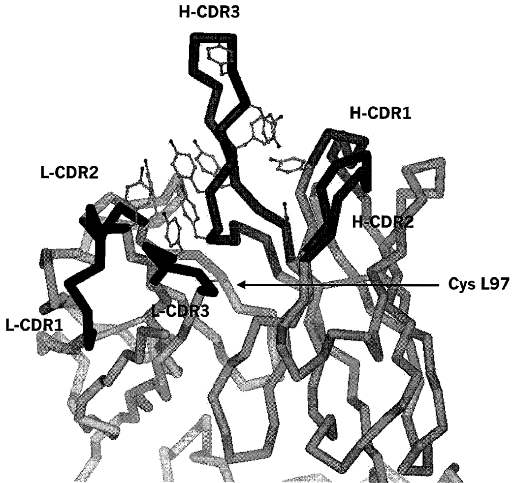
Figure 1. X-ray structure of AIN457 Fab
