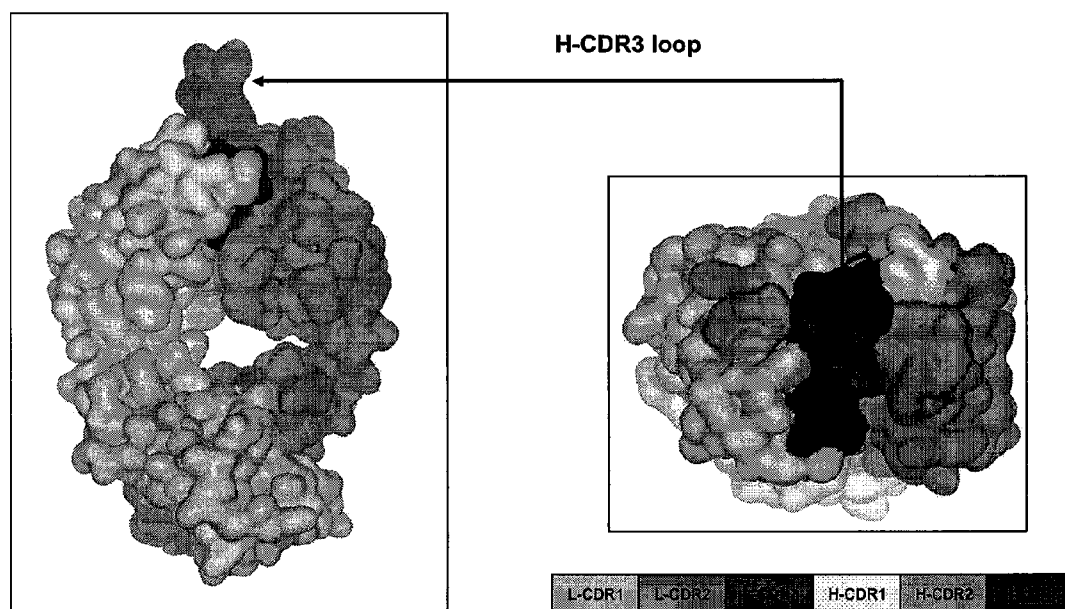
Figure 2. X-ray structure of AIN457 Fab, overall view
