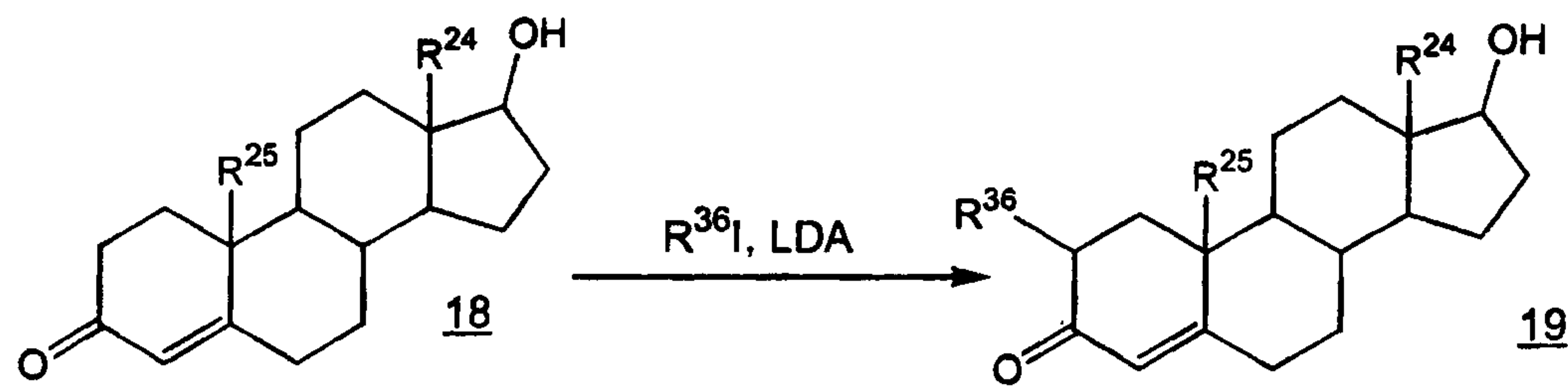
Scheme 13
