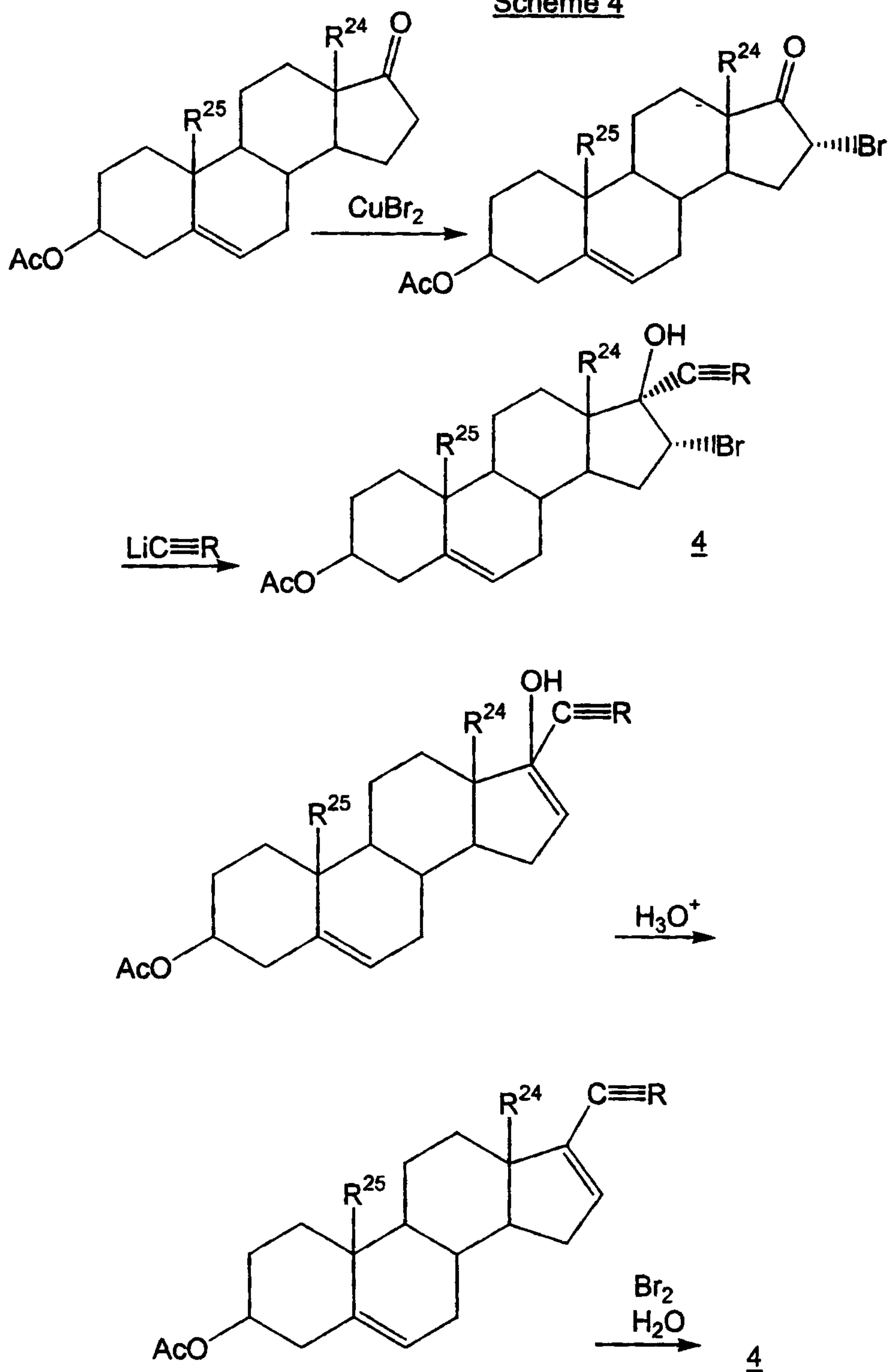
Scheme 4
