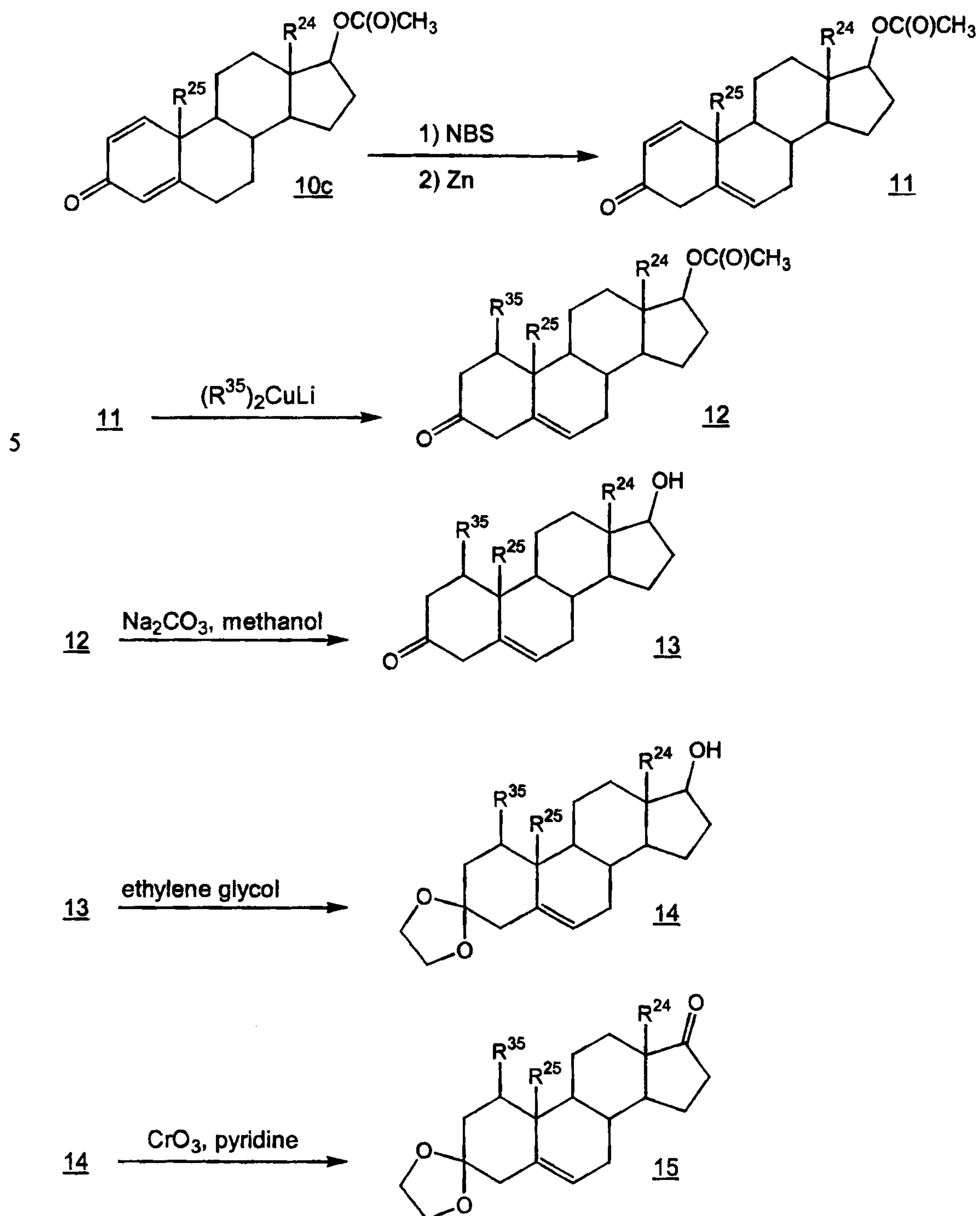
Scheme 11
