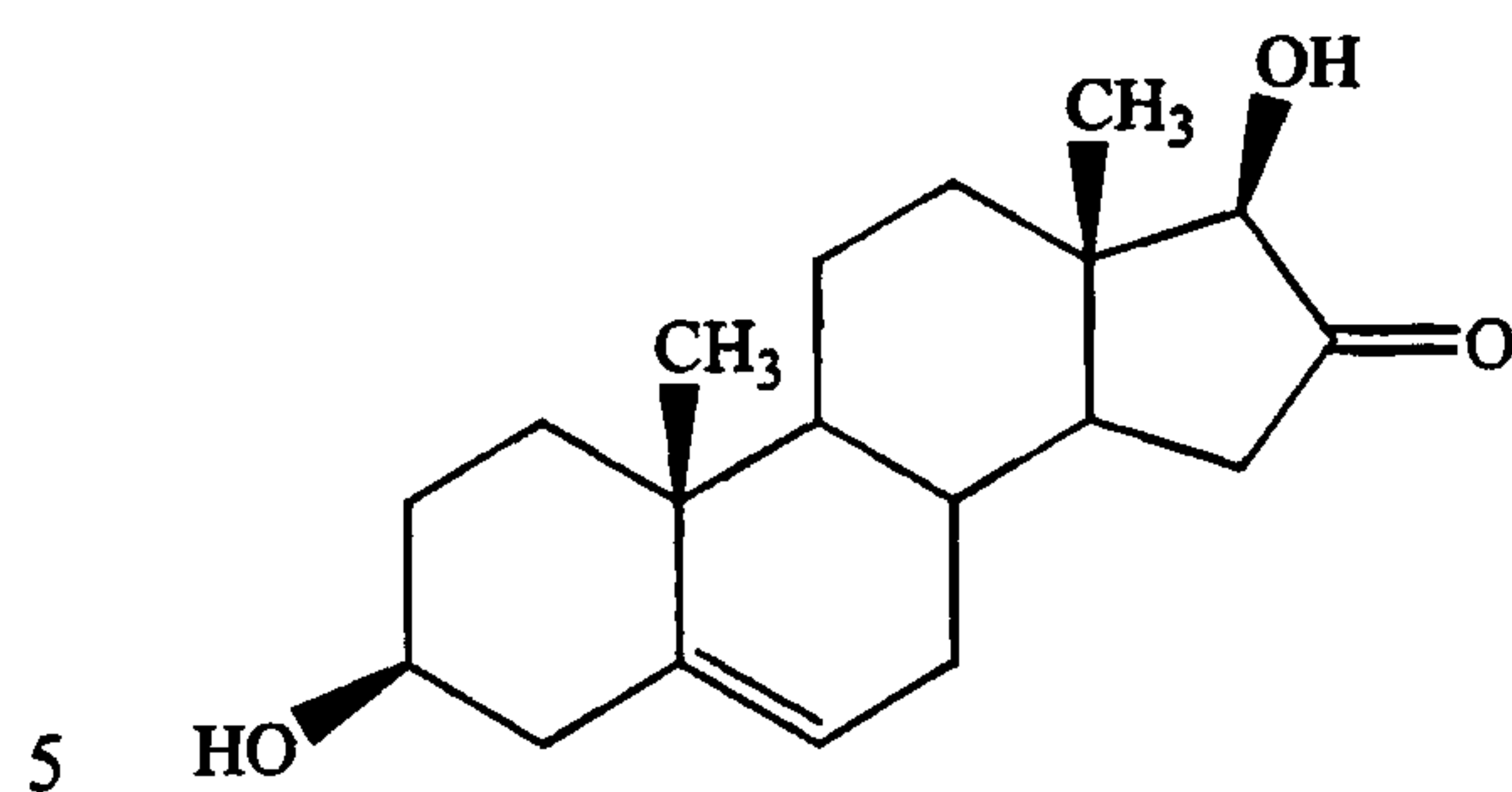
compound 8
