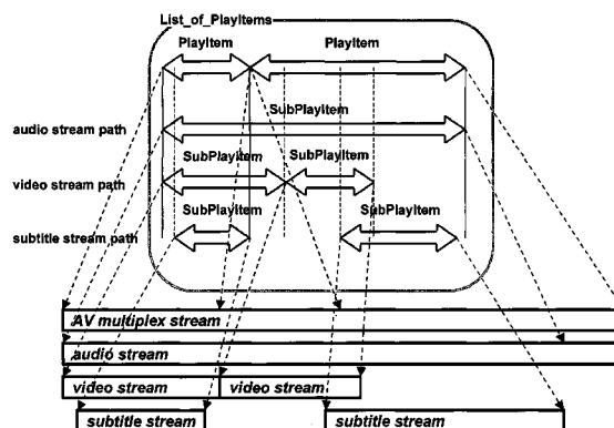
List_of_PlayItems Example
