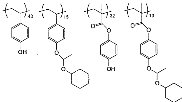
(RB-1) Mw 2500 Mw/Mn 1.30
