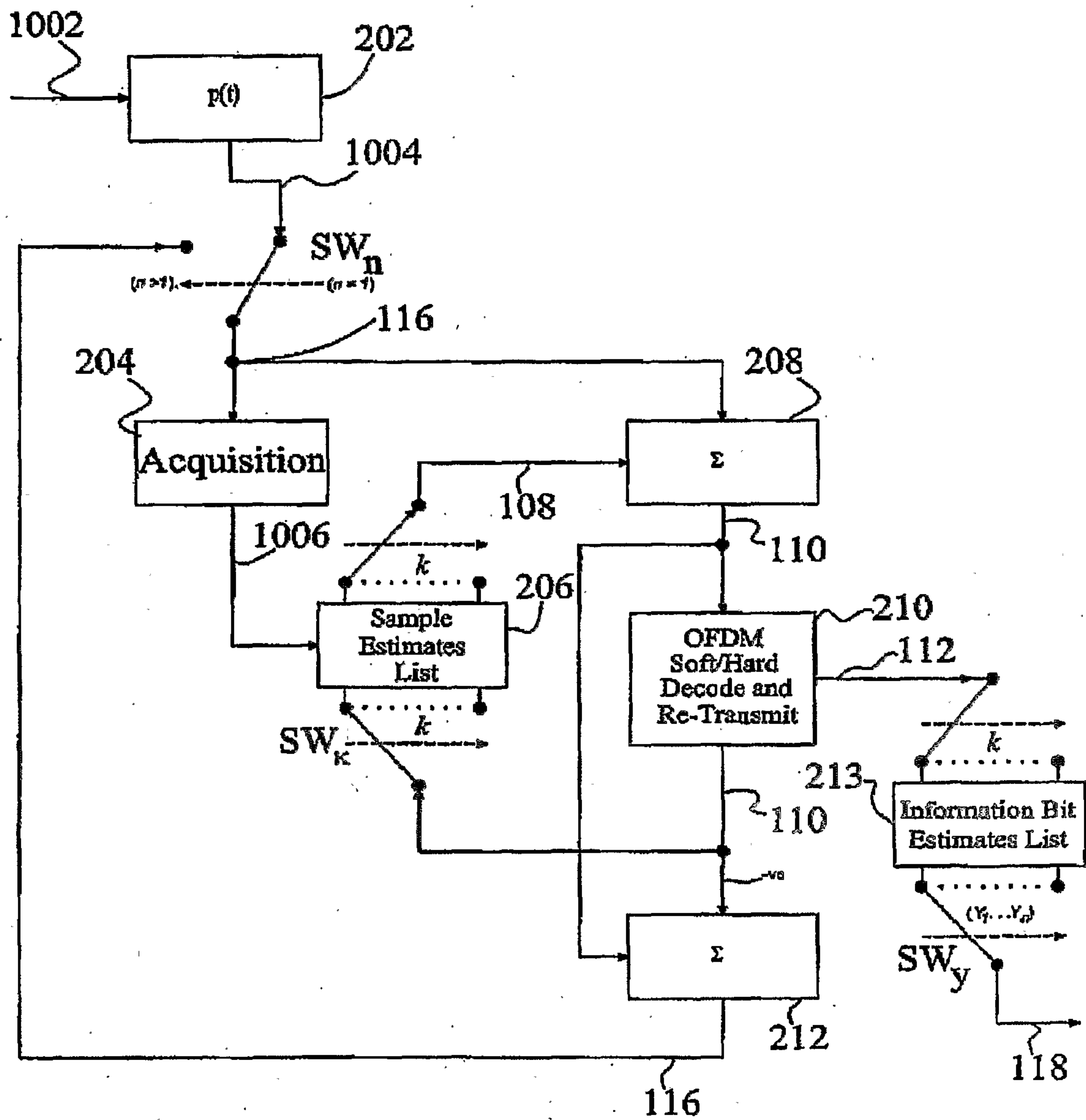
Iterative Interference Canceling Receiver Structure
