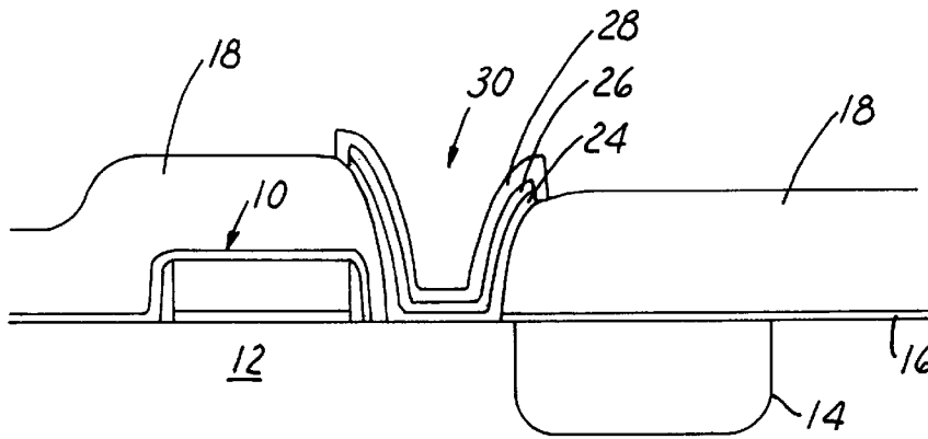
(PRIOR ART) FIG. 5
