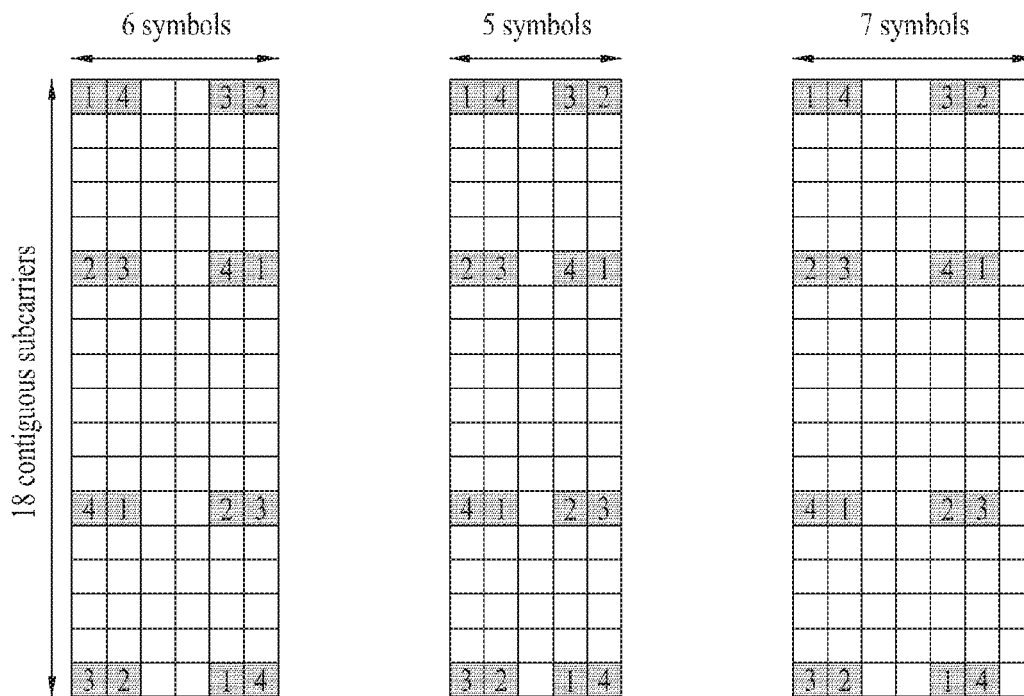
Pilot patterns on streams 0 ~ 3 for 4 data streams
