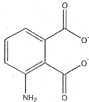
Aminophthalate ion
