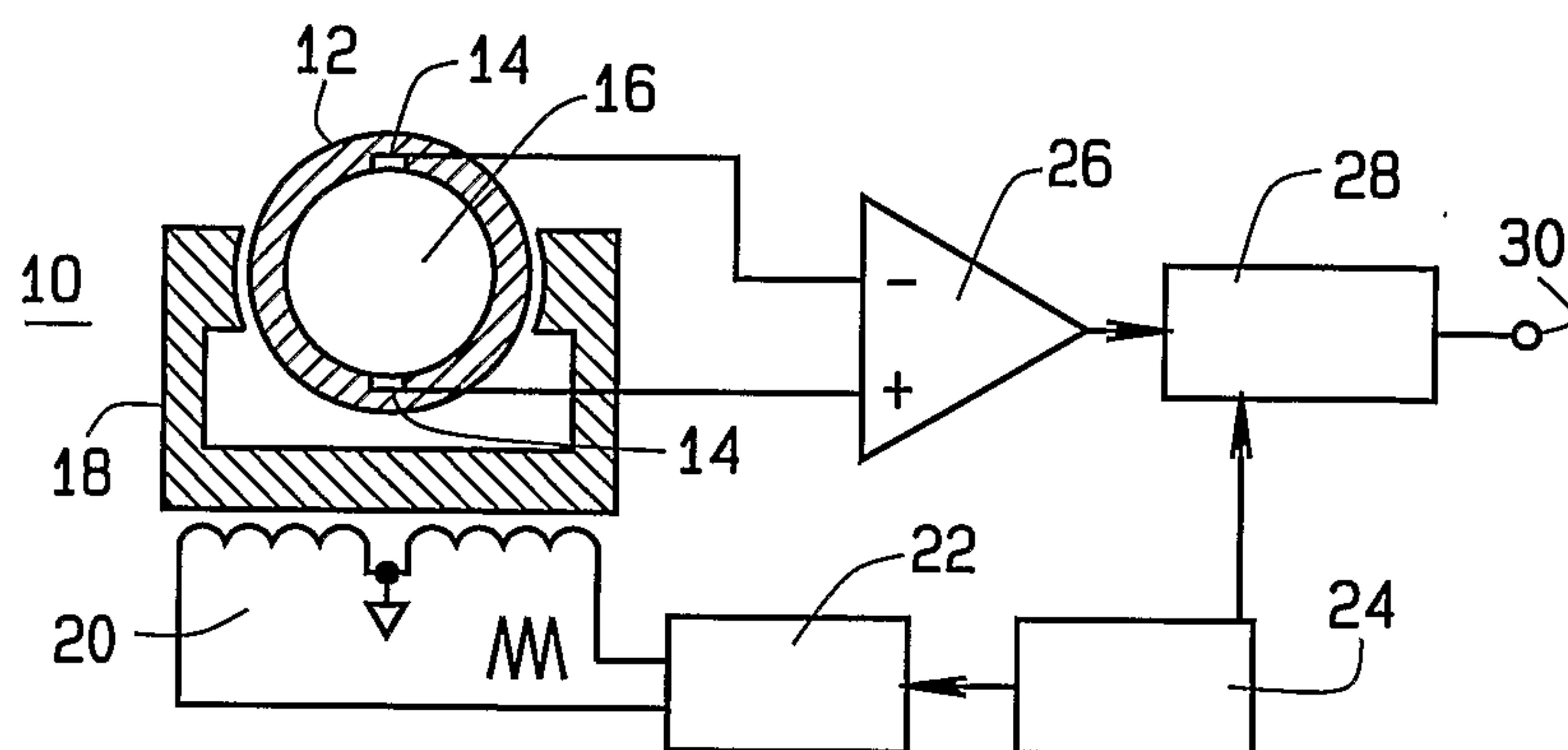
FIG. 1 PRIOR ART
