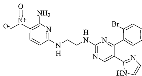
Compound 1:
